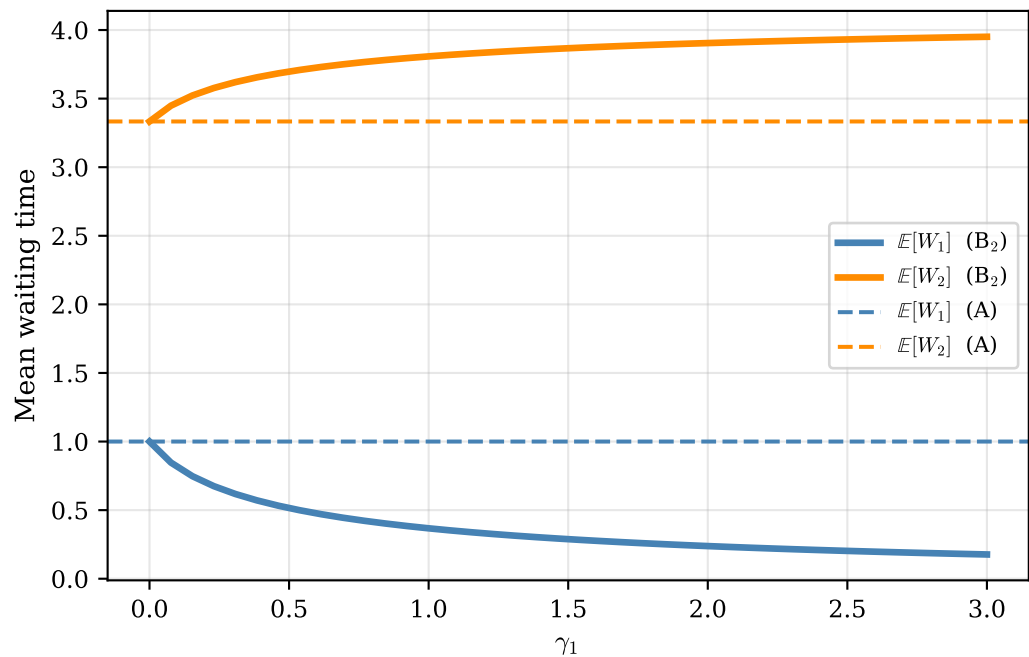
Model B_2 : mean waiting times vs \gamma_1
