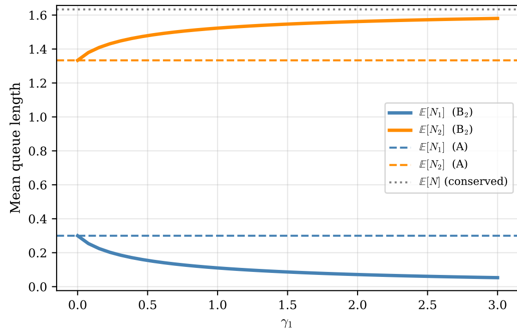
Model B_2 : mean queue lengths vs \gamma_1
