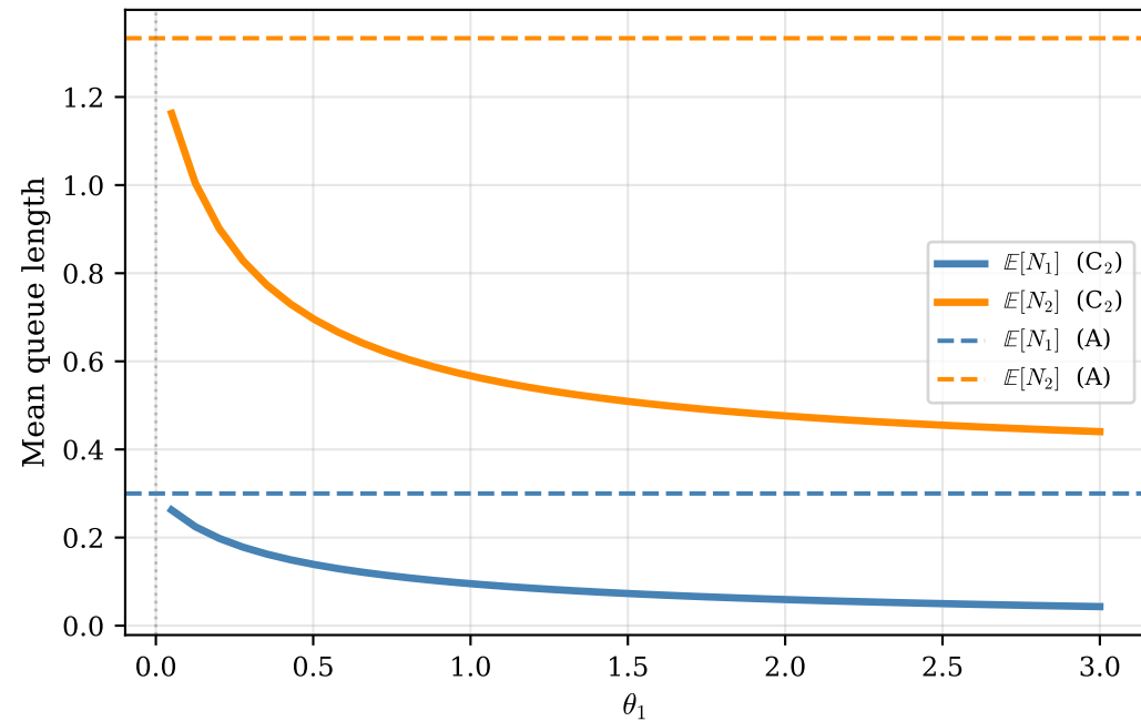
Model C 2 : mean queue lengths vs \theta_1
