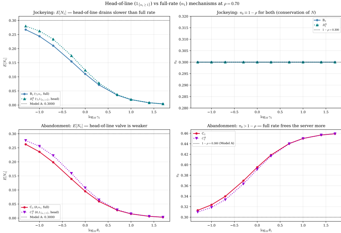
Figure 17: Head-of-line ( \mathbf{1}_{\{n_1 \geq 1\}} ) versus full-rate ( n_1 ) mechanisms at \rho = 0.70 ( \lambda_1 = 0.3 , \lambda_2 = 0.4 , \mu = 1 ). Top row, jockeying: E[N_1] and \pi_0 for B_2 (full) versus B_2^H (head-of-line). The head-of-line rate drains the priority queue more slowly, so E[N_1] stays above the B_2 curve, while \pi_0 \equiv 1 - \rho for both (jockeying conserves N , Corollaries 4, 6). Bottom row, abandonment: E[N_1] and \pi_0 for C_2 (full) versus C_2^H (head-of-line). The head-of-line valve is weaker, so C_2^H retains a slightly longer priority queue and a slightly smaller idle gain than C_2 , both models exceeding the 1 - \rho baseline (Corollaries 5, 7).
