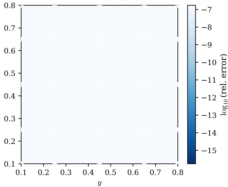
Model A (valid everywhere)
