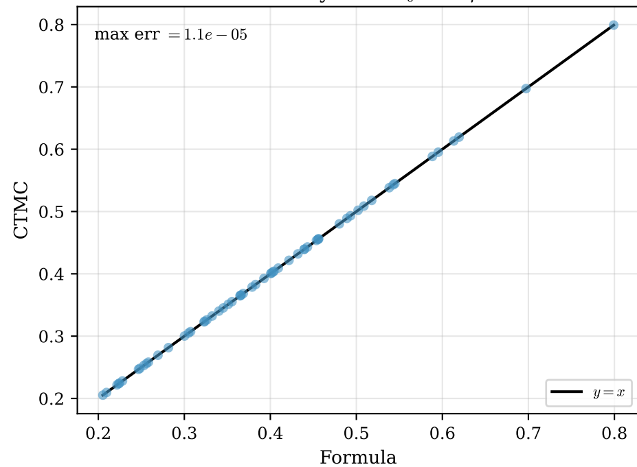
Corollary~C 2 — \pi_0
