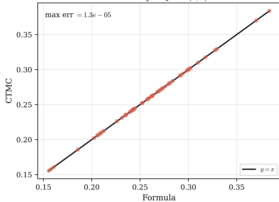
Corollary~C 2 — \pi(0, 0)
