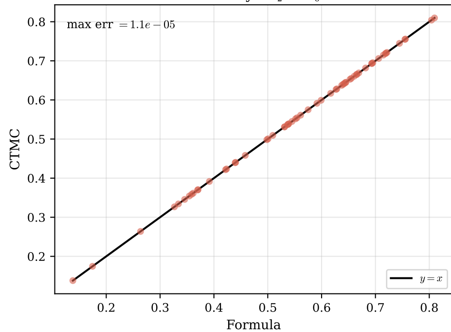
Corollary~C 2 — \pi_0
