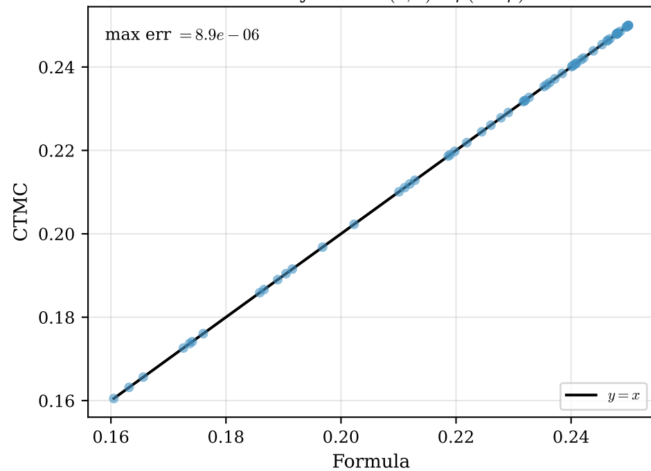
Corollary~C 2 — \pi(0, 0)
