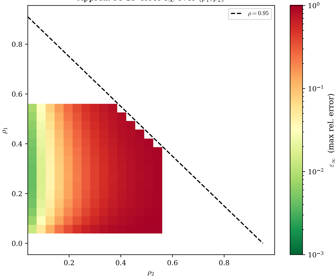
Approx. PPGF error \varepsilon_\infty over (\rho_1, \rho_2)
