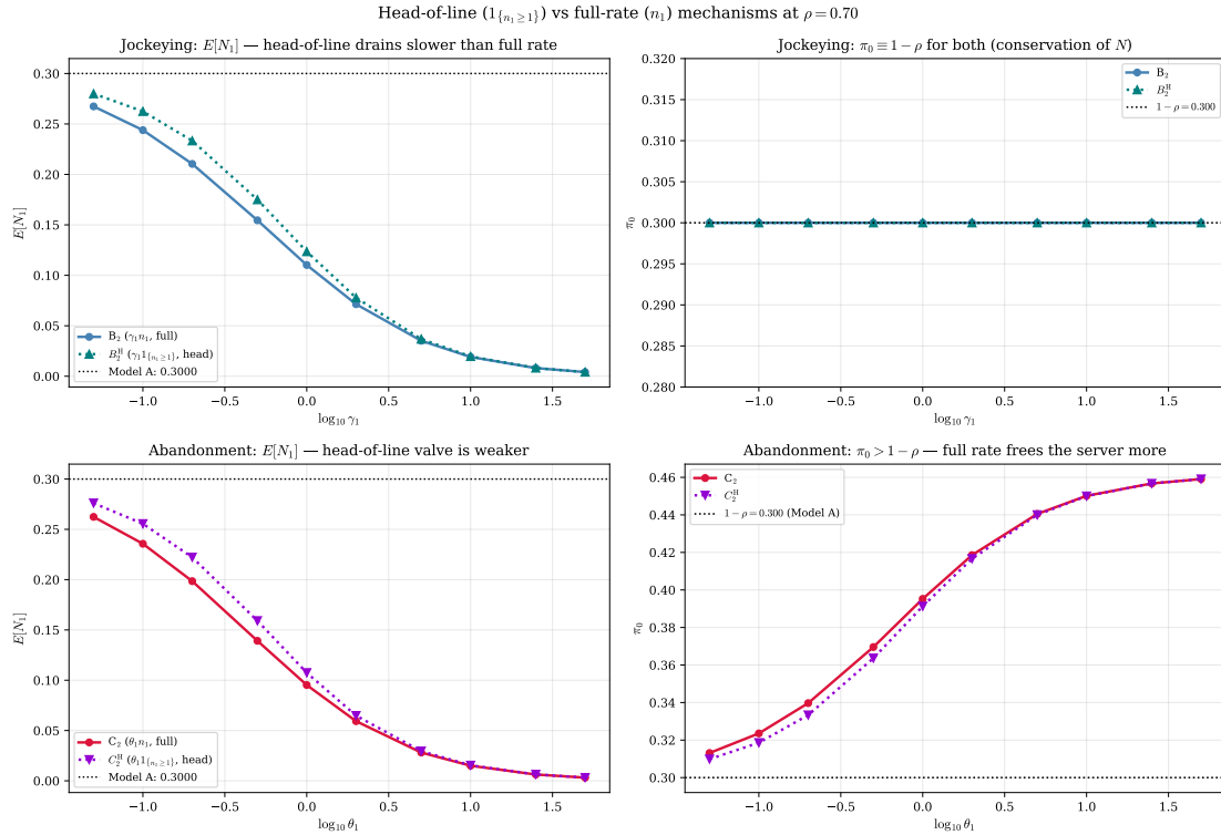
Figure 27: Head-of-line ( \mathbf{1}_{\{n_1 \geq 1\}} ) versus full-rate ( n_1 ) mechanisms at \rho = 0.70 ( \lambda_1 = 0.3 , \lambda_2 = 0.4 , \mu = 1 ). Top row, jockeying : \mathbb{E}[N_1] and \pi_0 for B_2 (full) versus B_2^H (head-of-line). The head-of-line rate drains the priority queue more slowly, so \mathbb{E}[N_1] stays above the B_2 curve, while \pi_0 \equiv 1 - \rho for both (jockeying conserves N , Corollaries 3, 5). Bottom row, abandonment : \mathbb{E}[N_1] and \pi_0 for C_2 (full) versus C_2^H (head-of-line). The head-of-line valve is weaker, so C_2^H retains a slightly longer priority queue and a slightly smaller idle gain than C_2 , both models exceeding the 1 - \rho baseline (Corollaries 4, 6).
