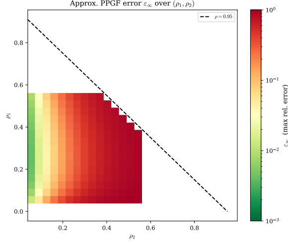
Figure 15: Max relative error \varepsilon_\infty of the approximate PPGF \tilde{P}_{\text{app}}(y, n) = (1 - \rho)\rho[\tilde{y}^*(y)]^n as a function of (\rho_1, \rho_2) . Colour convention (shared with the \mathbb{E}[N_1] heatmap, Figure 10): green marks the accurate regime ( \varepsilon_\infty < 3\% ) and red the inaccurate one—green favourable, red unfavourable, in the same direction across both maps. The approximation is reliable only when the priority class carries most of the offered load ( \rho_1/\rho \gtrsim 0.6 ) and the system is not heavily loaded ( \rho \lesssim 0.6 ).
