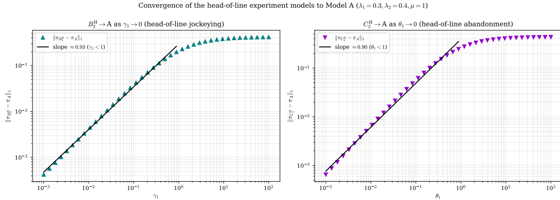
Figure 32: Convergence of the head-of-line experiment models to Model-A ( \lambda_1 = 0.3, \lambda_2 = 0.4, \mu = 1 ). Left : log-log plot of \|\pi_{B_2^H} - \pi_A\|_1 against \gamma_1 , with the fitted first-order slope. Right : \|\pi_{C_2^H} - \pi_A\|_1 against \theta_1 , likewise first-order. Both head-of-line variants approach the baseline at the same order as their full-rate counterparts B_2 and C_2 .
