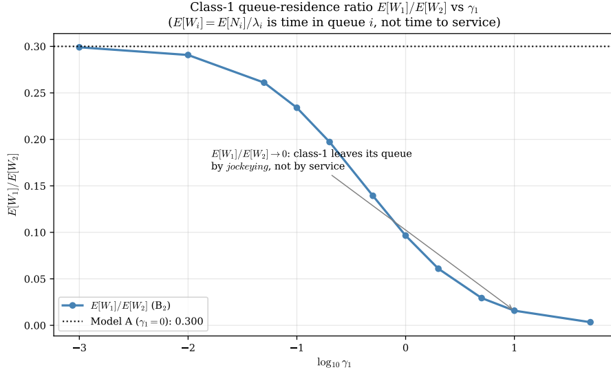
Figure 22: Class-1 queue-residence ratio \mathbb{E}[W_1]/\mathbb{E}[W_2] versus \gamma_1 at \rho = 0.70 , with the Model-A value dotted. The ratio decreases toward zero because \mathbb{E}[W_1] = \mathbb{E}[N_1]/\lambda_1 measures time spent in the class-1 queue, which the jockeying drain \gamma_1 \mathbb{E}[N_1] collapses; it does not measure time to service.
