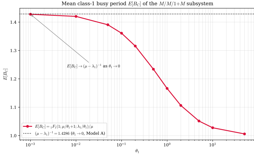
Figure 26: Mean class-1 busy period \mathbb{E}[B_C] of the M/M/1+M subsystem versus \theta_1 , computed in closed form from \mathbb{E}[B_C] = {}_1F_1(1; \mu/\theta_1 + 1; \lambda_1/\theta_1)/\mu (cf. (11.1)). The horizontal asymptote is the Model-A busy period (\mu - \lambda_1)^{-1} = 1.4286 , attained as \theta_1 \rightarrow 0^+ (Corollary 4 limit).
