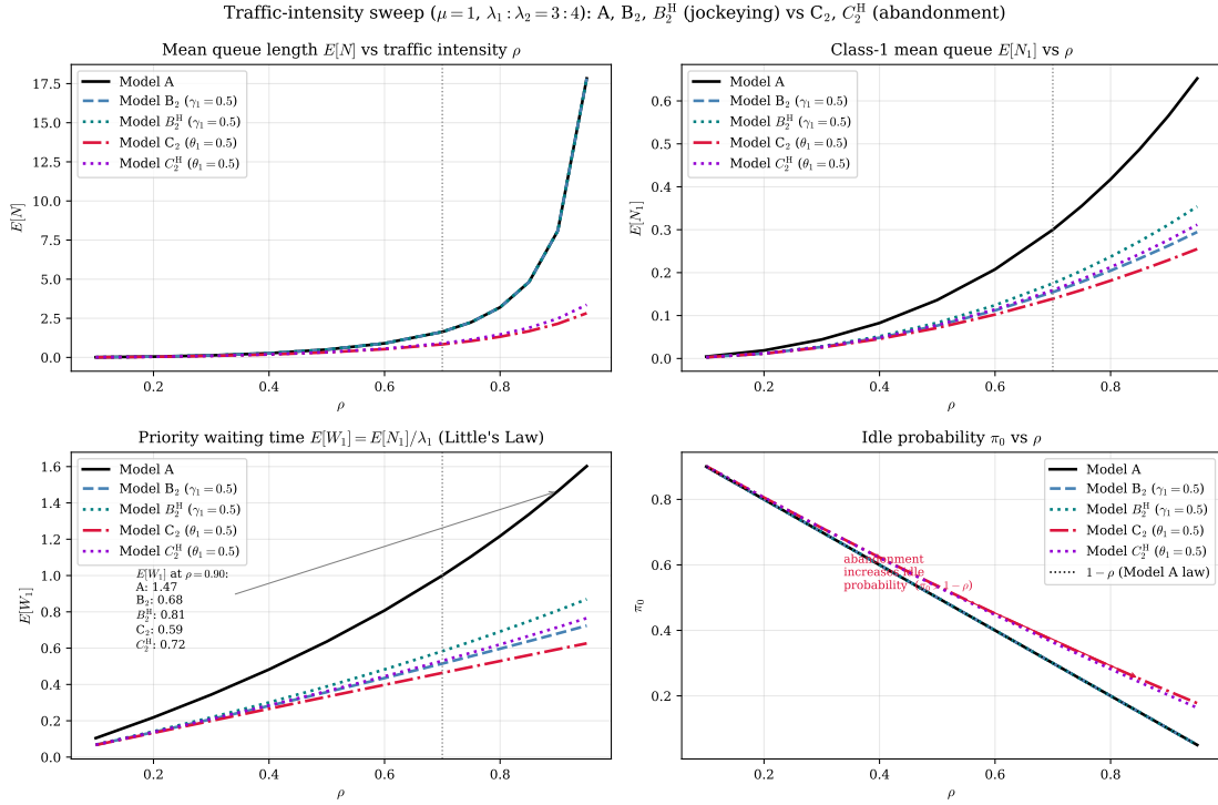
Figure 9: Performance versus traffic intensity \rho for the five solved models — the baseline A, the jockeying pair B_2 , B_2^H ( \gamma_1 = 0.5 ), and the abandonment pair C_2 , C_2^H ( \theta_1 = 0.5 ) — at \mu = 1 and \lambda_1:\lambda_2 = 3:4 ; the vertical line marks the canonical \rho = 0.70 . Top-left : total queue \mathbb{E}[N] — A, B_2 and B_2^H coincide because jockeying conserves N (Corollaries 1, 5), while C_2 and C_2^H lie strictly below because abandonment removes customers ( C_2^H by less). Top-right : priority queue \mathbb{E}[N_1] — the head-of-line variants drain it less than their full-rate cousins. Bottom-left : priority waiting time \mathbb{E}[W_1] . Bottom-right : idle probability \pi_0 , with the 1 - \rho law (Models A, B_2 , B_2^H ) shown dotted; C_2 and C_2^H sit above it for every \rho , as predicted by Corollaries 4, 6.
