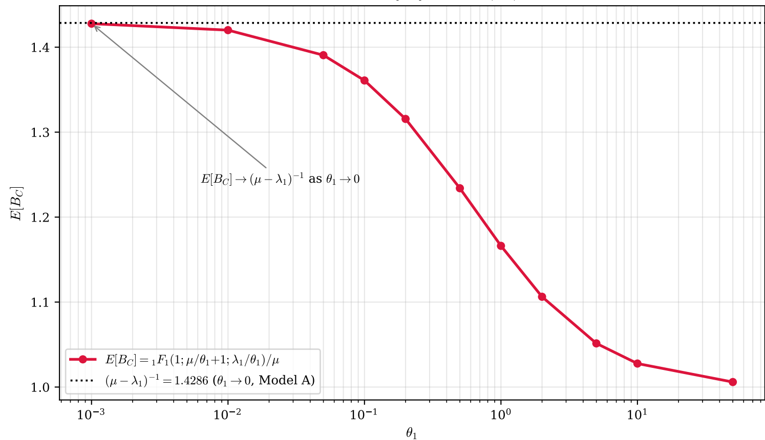
Mean class-1 busy period E[B_C] of the M/M/1+M subsystem
