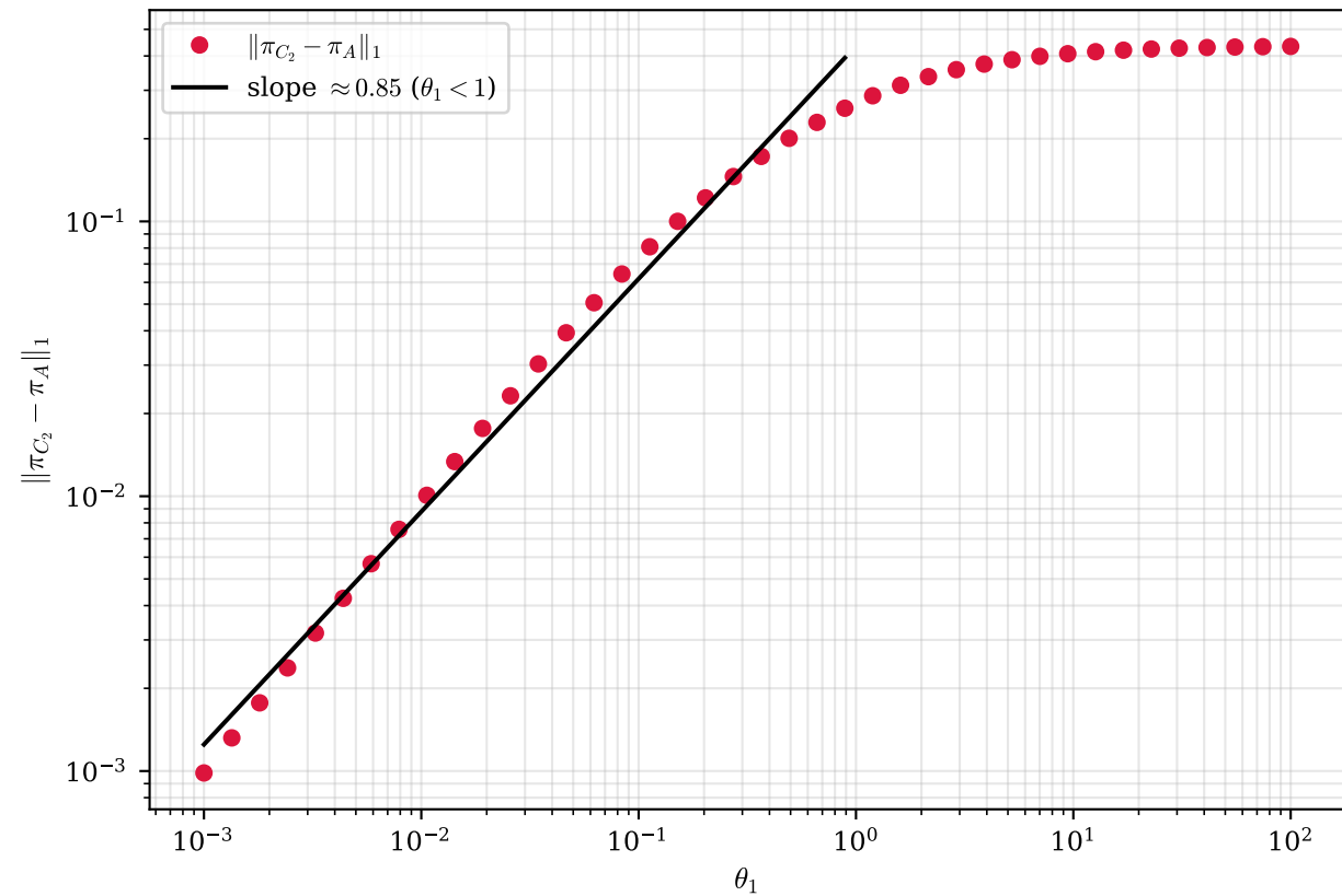
L_1 convergence of C_2 to A as \theta_1 \rightarrow 0
