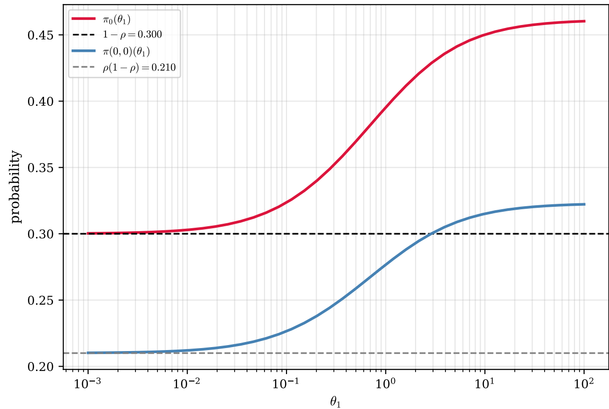
\pi_0, \pi(0,0) \rightarrow Model A values as \theta_1 \rightarrow 0
