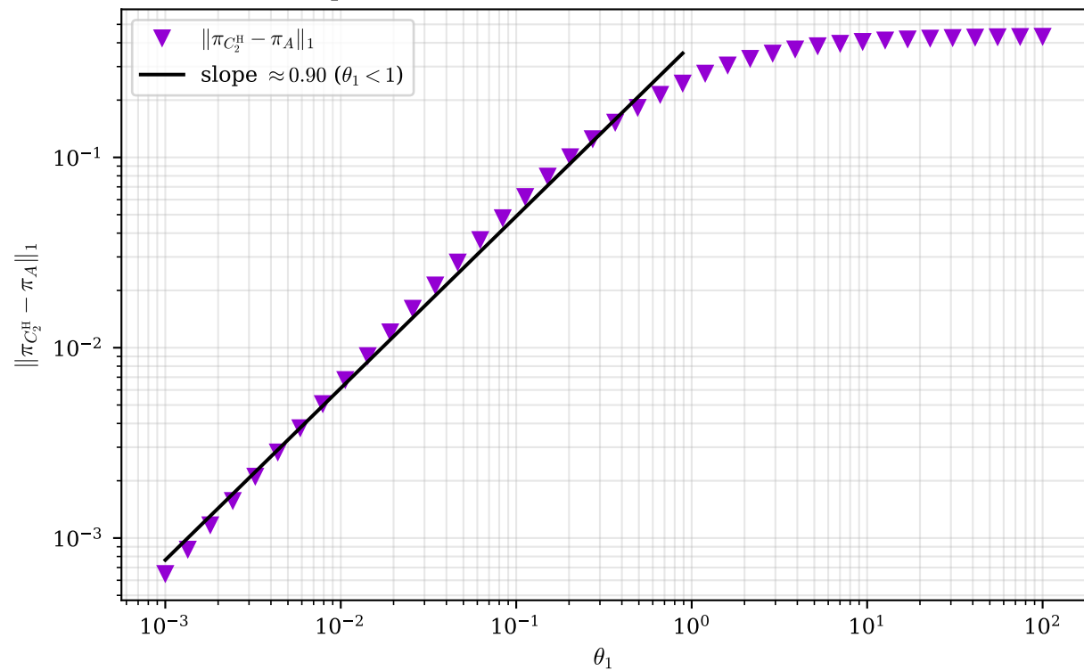
C_2^H \rightarrow A as \theta_1 \rightarrow 0 (head-of-line abandonment)
