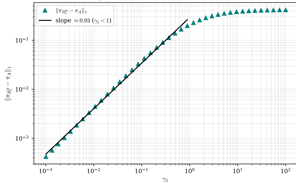
B_2^H \rightarrow A as \gamma_1 \rightarrow 0 (head-of-line jockeying)
