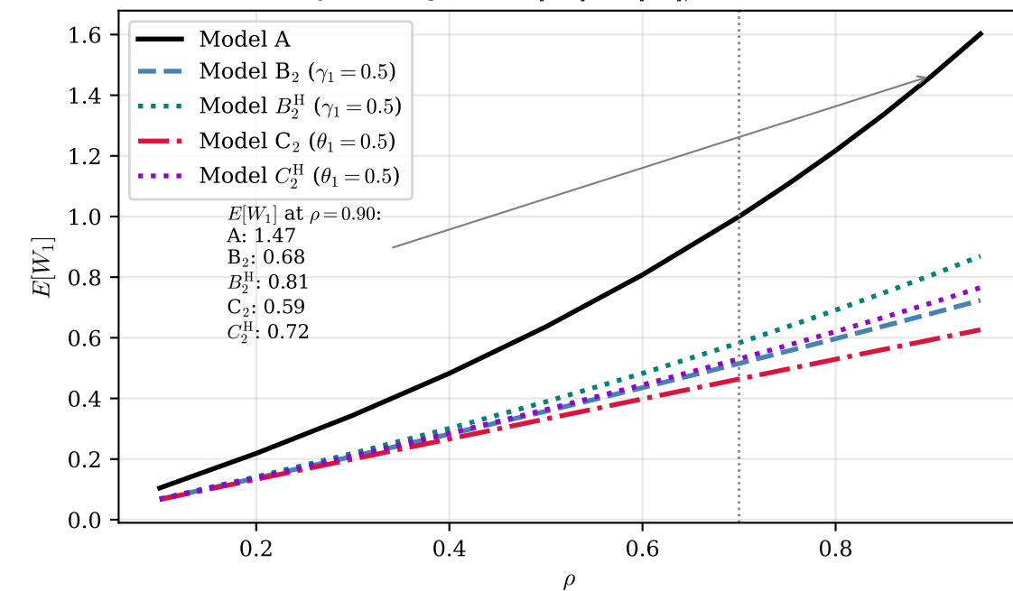
Priority waiting time E[W_1] = E[N_1]/\lambda_1 (Little's Law)
