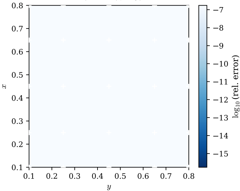
Model A (valid everywhere)
