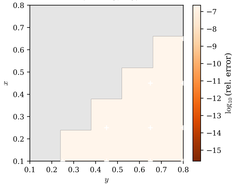
Model B_2 ( \gamma_1 = 0.5 , valid x < y )
