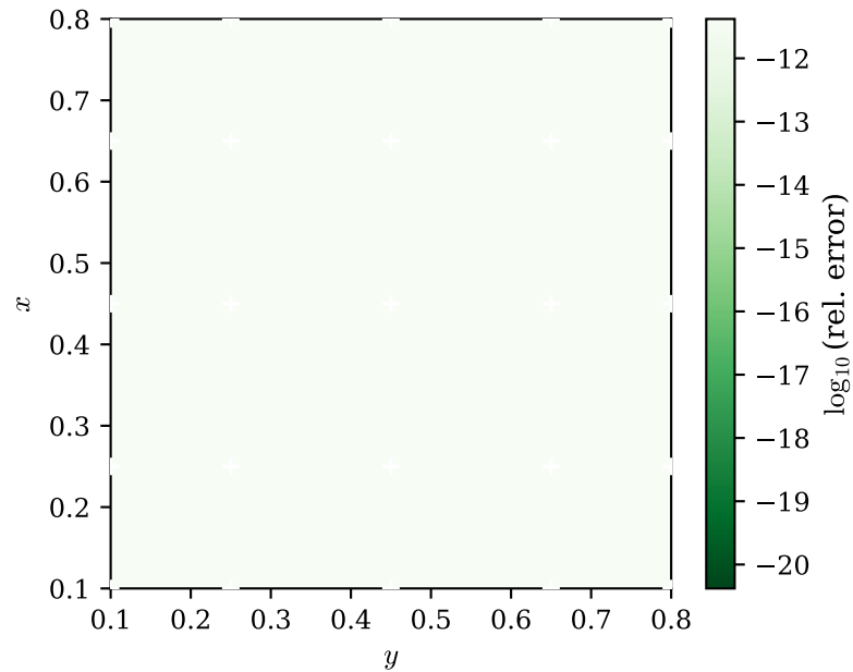
Model C_2 ( \theta_1 = 0.5 , valid everywhere)
