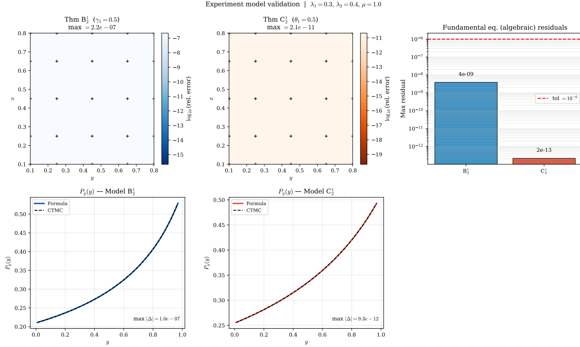
Figure 23: Validation of Models B_2^1 and C_2^1 . Top row, left and centre : relative error |P_{\text{formula}}(x, y) - P_{\text{CTMC}}(x, y)| / |P_{\text{CTMC}}(x, y)| on the 5 \times 5 test grid. Top row, right : maximum relative residual of the algebraic fundamental equation for each model — both well below the 10^{-6} tolerance. Bottom row : boundary function P_y(y) = P(0, y) comparing the rational closed-form formula against the CTMC.
