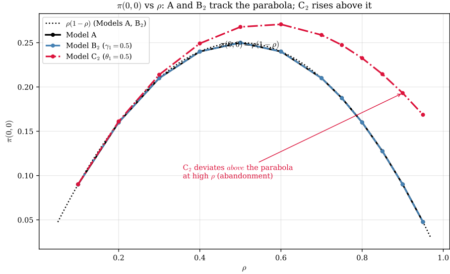
Figure 9: \pi(0,0) versus \rho . Models A and B_2 lie exactly on the parabola \rho(1 - \rho) (Corollary 2 and Corollary 4: jockeying preserves N , hence the busy-but-empty probability), whereas C_2 rises strictly above it — abandonment inflates \pi(0,0) through the enlarged idle probability \pi(0,0) = \rho \pi_0 of Corollary 5.
