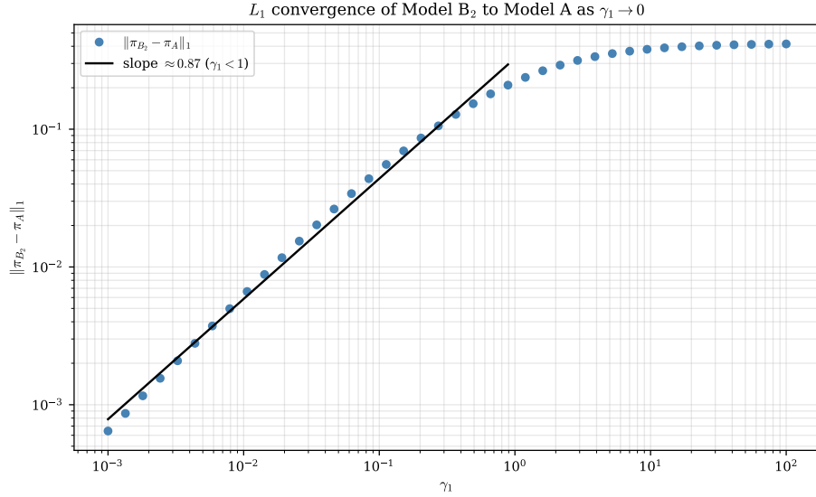
Figure 28: Convergence of Model B_2 to Model A as \gamma_1 \rightarrow 0^+ . The log-log L_1 distance has fitted slope 0.87 over \gamma_1 < 1 , again first-order, even though the B_2 limit is singular in the ODE (the \gamma_1 \rightarrow 0 limit is non-uniform in the analytic continuation, but the stationary distribution responds at first order).
