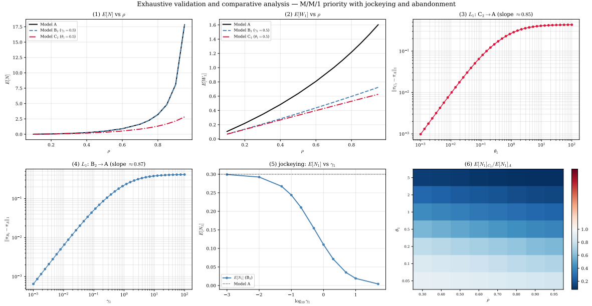
Figure 30: Synoptic dashboard of the numerical study: (1) \mathbb{E}[N] and (2) \mathbb{E}[W_1] versus \rho for all models; (3) L_1 convergence C_2 \rightarrow A and (4) B_2 \rightarrow A ; (5) the jockeying effect on \mathbb{E}[N_1] ; and (6) the \mathbb{E}[N_1]_{C_2}/\mathbb{E}[N_1]_A heatmap over (\rho, \theta_1) . Together these panels summarise the two central findings: jockeying redistributes delay at fixed total work, while abandonment reduces total work at a throughput cost.
