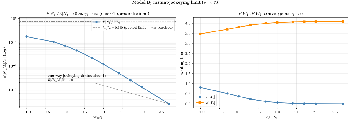
Figure 29: Model B_2 in the strong-jockeying regime \gamma_1 \rightarrow \infty at \rho = 0.70 . Left: \mathbb{E}[N_1]/\mathbb{E}[N_2] \rightarrow 0 (note the logarithmic ordinate): one-way jockeying is absorbing, so the class-1 queue is drained completely. Right: \mathbb{E}[W_1] \rightarrow 0 while \mathbb{E}[W_2] saturates as \mathbb{E}[N_2] \rightarrow \mathbb{E}[N]_A .
