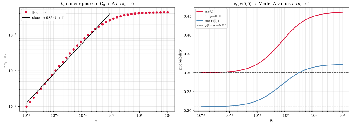
Figure 26: Convergence of Model C_2 to Model A as \theta_1 \rightarrow 0^+ ( \lambda_1 = 0.3 , \lambda_2 = 0.4 , \mu = 1 ). Left : log-log plot of \|\pi_{C_2} - \pi_A\|_1 against \theta_1 , with a fitted slope of 0.85 over \theta_1 < 1 . Right : \pi_0(\theta_1) and \pi(0, 0)(\theta_1) relaxing onto the Model-A values 1 - \rho = 0.30 and \rho(1 - \rho) = 0.21 as \theta_1 \rightarrow 0 .
