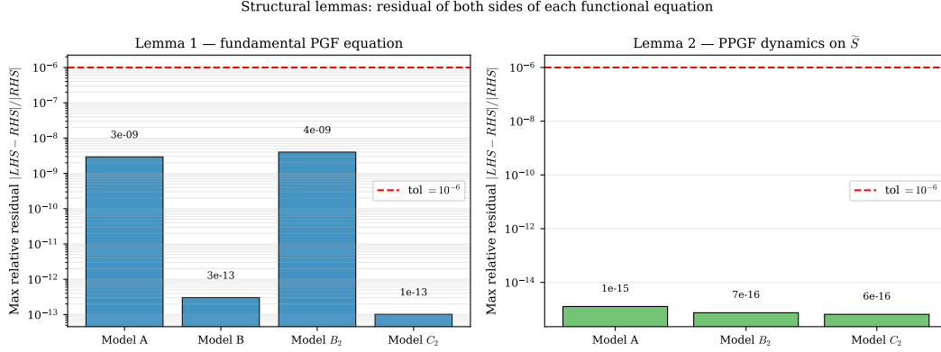
Figure 17: Lemma validation. Left : max relative residual of the fundamental PGF equation (Lemma 1) for each model variant on a 5 \times 5 interior grid. Right : max relative residual of the PPGF dynamics recurrence (Lemma 2) over n \in \{1, \dots, 15\} and y \in [0.05, 0.90] . All values lie well below the 10^{-6} tolerance (red dashed line).
