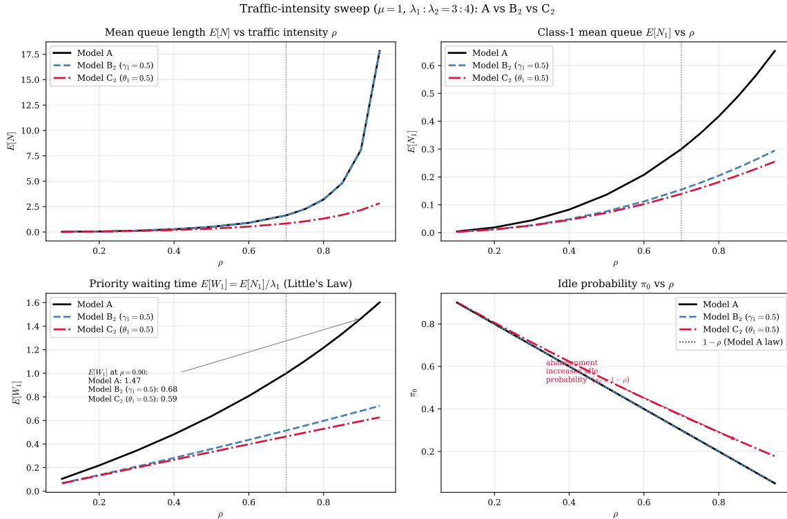
Figure 8: Performance versus traffic intensity \rho for Models A , B_2 ( \gamma_1 = 0.5 ) and C_2 ( \theta_1 = 0.5 ), at \mu = 1 and \lambda_1:\lambda_2 = 3:4 ; the vertical line marks the canonical \rho = 0.70 . Top-left : total queue \mathbb{E}[N] — A and B_2 coincide because jockeying conserves N (Corollary 2), while C_2 lies strictly below because abandonment removes customers. Top-right : priority queue \mathbb{E}[N_1] . Bottom-left : priority waiting time \mathbb{E}[W_1] . Bottom-right : idle probability \pi_0 , with the 1 - \rho law (Model A/B_2 ) shown dotted; C_2 sits above it for every \rho , as predicted by Corollary 5.
