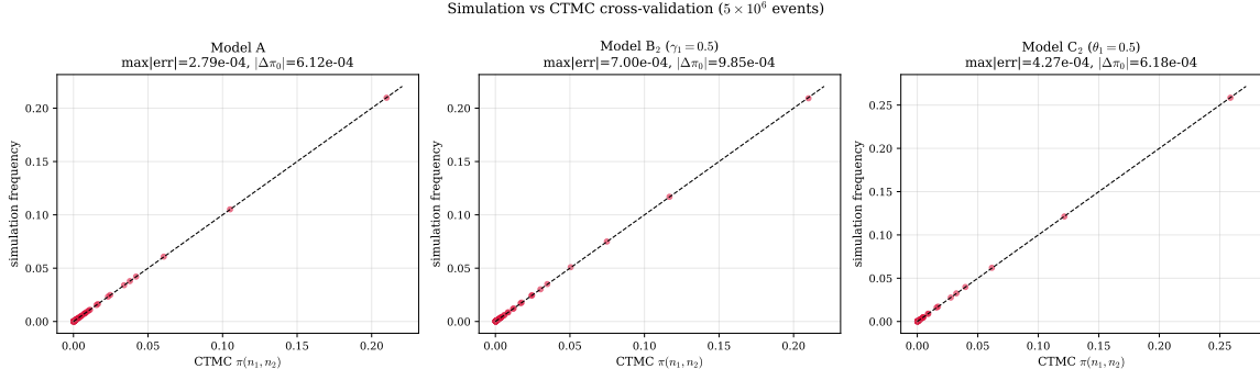
Figure 25: Simulation versus exact CTMC for Models A , B_2 ( \gamma_1 = 0.5 ) and C_2 ( \theta_1 = 0.5 ) at \lambda_1 = 0.3 , \lambda_2 = 0.4 , \mu = 1 . Each point is one state (n_1, n_2) ; the dashed line is y = x . The simulation uses 5 \times 10^6 events (lower precision than the CTMC), yet every point lies on the diagonal, with maximum absolute discrepancy below 10^{-2} for all three models.
