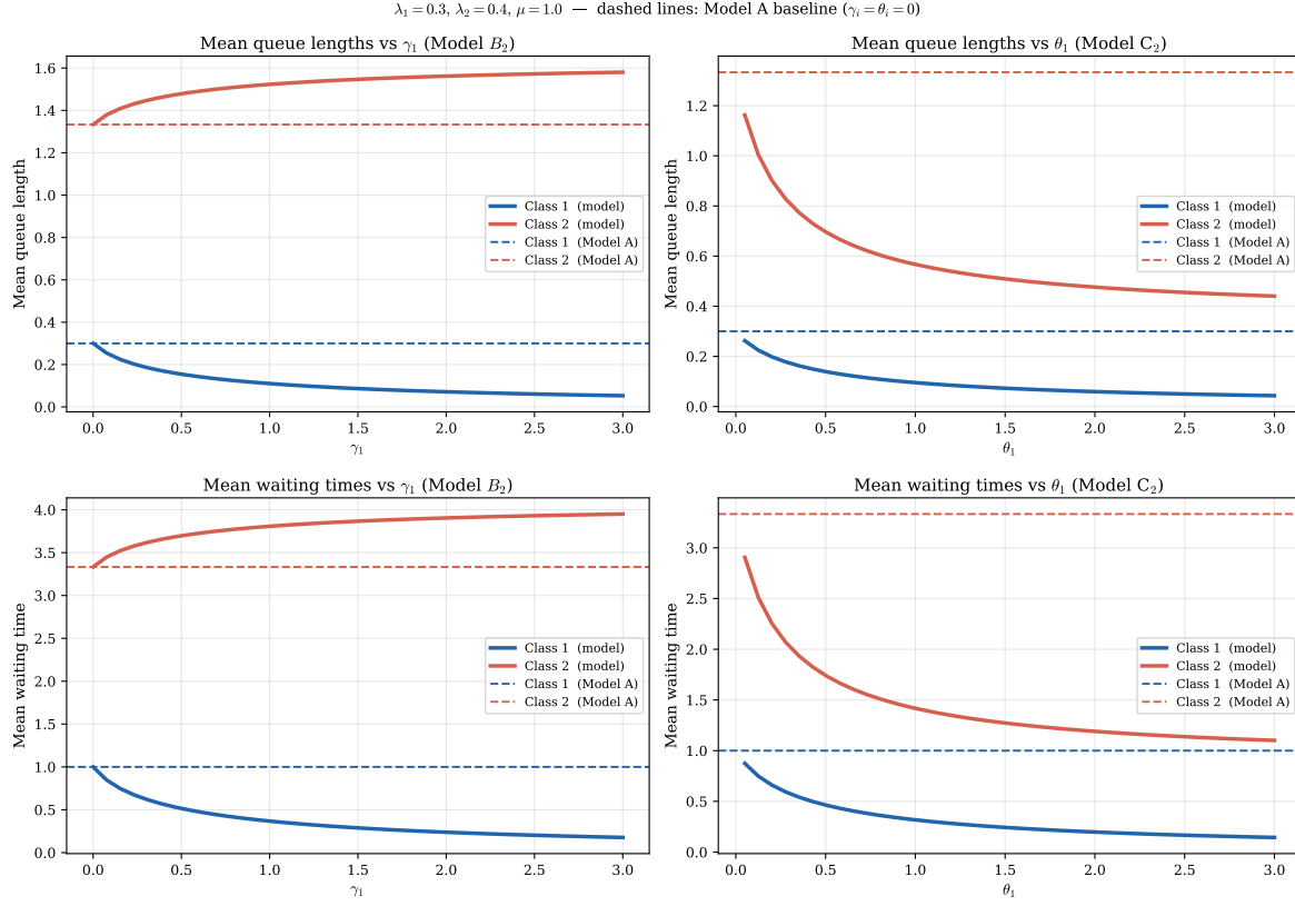
Figure 22: Mean queue lengths (top row) and mean waiting times (bottom row) for Models B_2 (left column) and C_2 (right column) as their respective mechanism parameters vary. Dashed lines indicate the Model A baseline.
