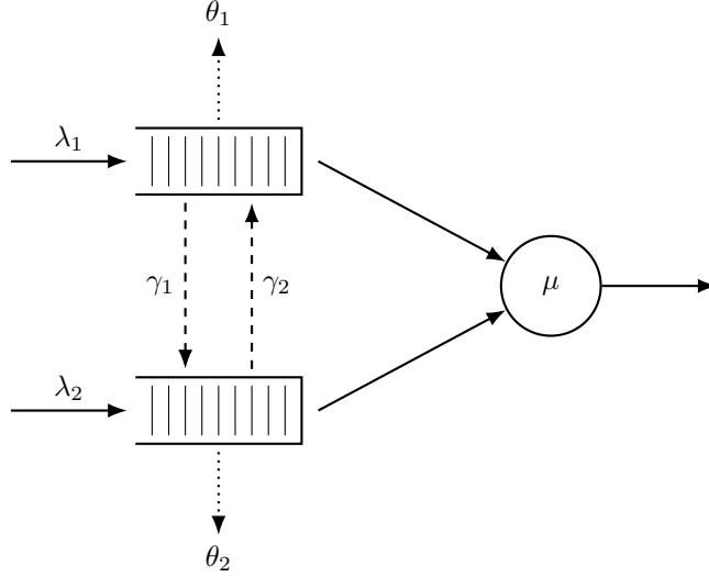
Figure 2: Queueing system with two parallel queues.
