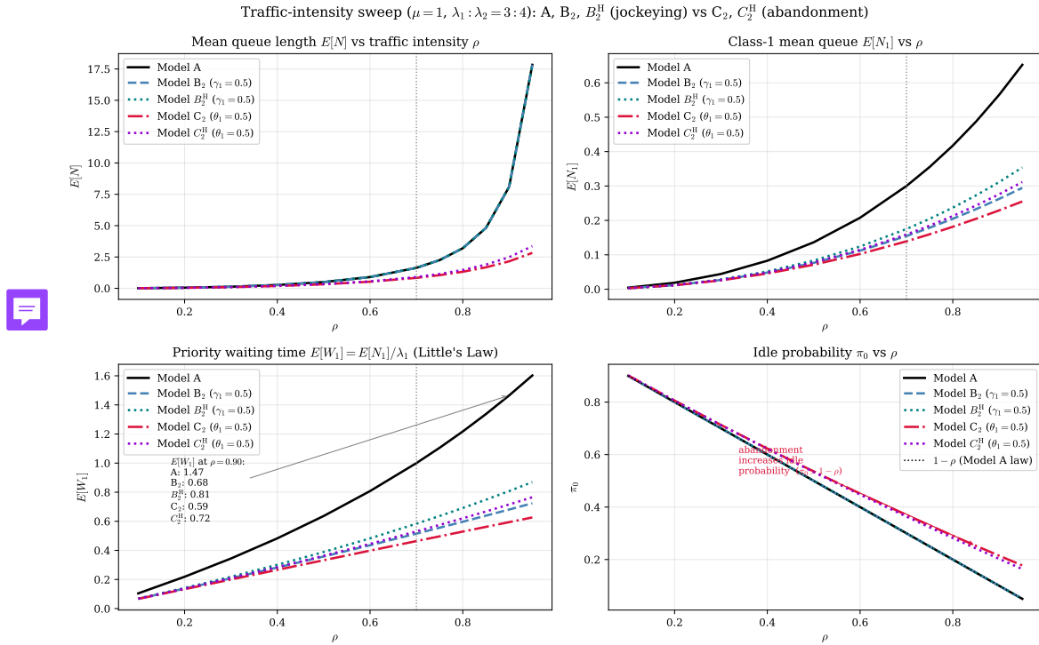
Figure 8: Performance versus traffic intensity \rho for the five solved models—the baseline A, the jockeying pair B_2 , B_2^H ( \gamma_1 = 0.5 ), and the abandonment pair C_2 , C_2^H ( \theta_1 = 0.5 )—at \mu = 1 and \lambda_1:\lambda_2 = 3:4 ; the vertical line marks the canonical \rho = 0.70 . Top-left : total queue \mathbb{E}[N] —A, B_2 and B_2^H coincide because jockeying conserves N (Corollaries 2, 6), while C_2 and C_2^H lie strictly below because abandonment removes customers ( C_2^H by less). Top-right : priority queue \mathbb{E}[N_1] —the head-of-line variants drain it less than their full-rate cousins. Bottom-left : priority waiting time \mathbb{E}[W_1] . Bottom-right : idle probability \pi_0 , with the 1 - \rho law (Models A, B_2 , B_2^H ) shown dotted; C_2 and C_2^H sit above it for every \rho , as predicted by Corollaries 5, 7.
