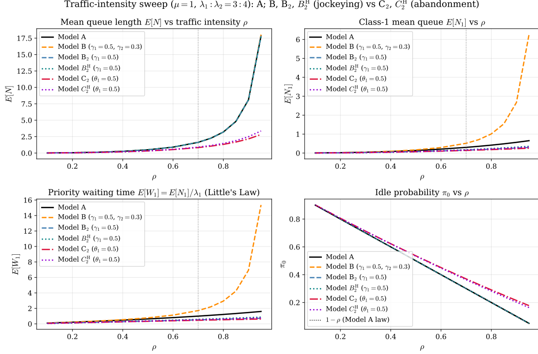
Figure 8: Performance versus traffic intensity \rho for the five solved models and the open Model- B —the baseline A , the jockeying models B ( \gamma_1 = 0.5, \gamma_2 = 0.3 ), B_2 and B_2^H ( \gamma_1 = 0.5 ), and the abandonment pair C_2 , C_2^H ( \theta_1 = 0.5 )— at \mu = 1 and \lambda_1:\lambda_2 = 3:4 ; the vertical line marks the canonical \rho = 0.70 . Top-left : total queue \mathbb{E}[N] — A , B , B_2 and B_2^H coincide because jockeying conserves N (Corollaries 3, 4, 7), while C_2 and C_2^H lie strictly below because abandonment removes customers ( C_2^H by less). Top-right : priority queue \mathbb{E}[N_1] —the head-of-line variants drain it less than their full-rate counterparts, and the two-way Model- B lengthens it. Bottom-left : priority waiting time \mathbb{E}[W_1] . Bottom-right : idle probability \pi_0 , with the 1 - \rho law (Models A , B , B_2 , B_2^H ) shown dotted; C_2 and C_2^H lie above it for every \rho , as predicted by Corollaries 6, 8.
