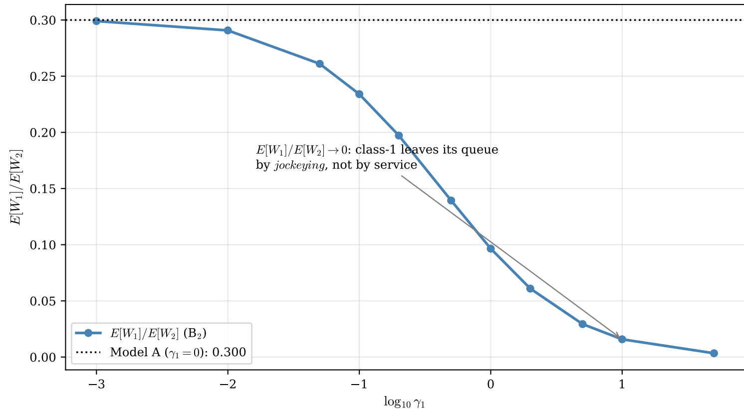
Class-1 queue-residence ratio E[W_1]/E[W_2] vs \gamma_1 ( E[W_i] = E[N_i]/\lambda_i is time in queue i , not time to service)
