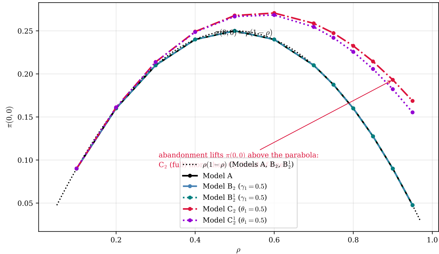
\pi(0,0) vs \rho : A, B_2 , B_2^1 track the parabola; C_2 , C_2^1 rise above
