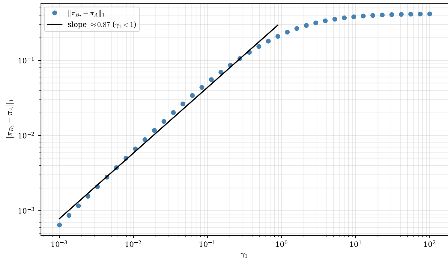
L_1 convergence of Model B_2 to Model A as \gamma_1 \rightarrow 0
