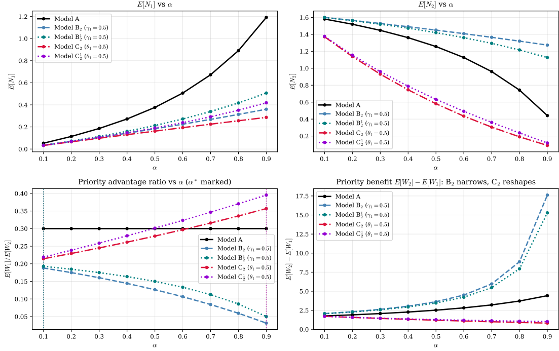
Class-asymmetry analysis ( \rho = 0.70 )
