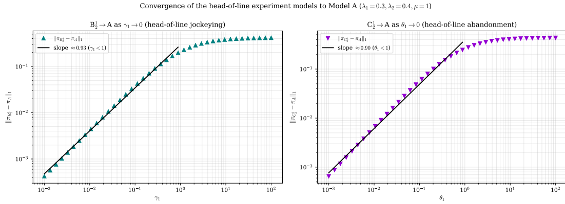
Figure 32: Convergence of the head-of-line experiment models to Model A ( \lambda_1 = 0.3, \lambda_2 = 0.4, \mu = 1 ). Left : log-log plot of \|\pi_{B_2^1} - \pi_A\|_1 against \gamma_1 , with the fitted first-order slope. Right : \|\pi_{C_2^1} - \pi_A\|_1 against \theta_1 , likewise first-order. Both head-of-line variants approach the baseline at the same order as their full-rate counterparts B_2 and C_2 .
