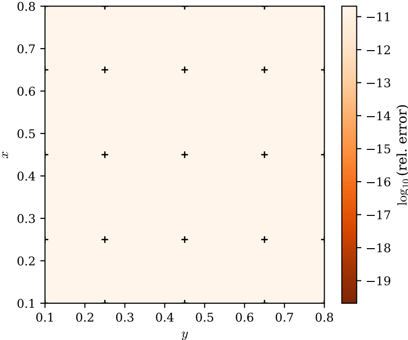
Thm C 2 1 ( \theta_1 = 0.5 ) max = 2.1e-11
