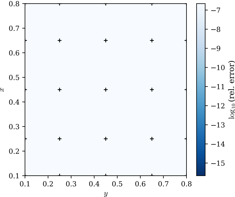
Thm B 2 1 ( \gamma_1 = 0.5 ) max = 2.2e-07
