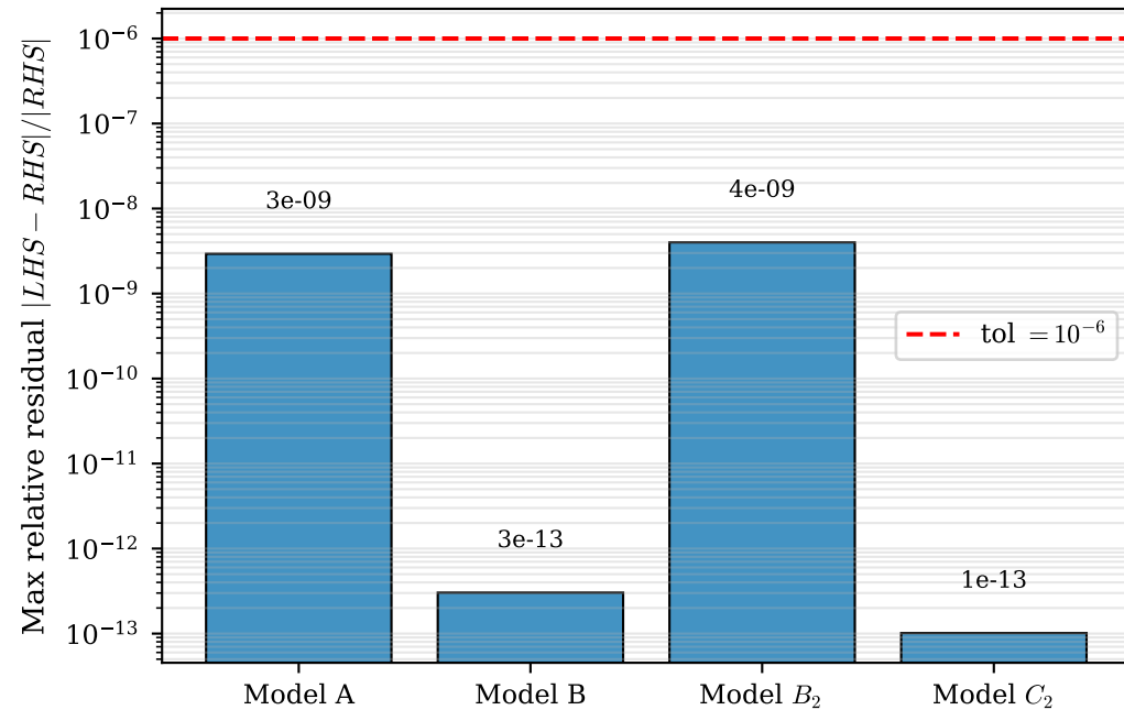
Lemma 1 — fundamental PGF equation
