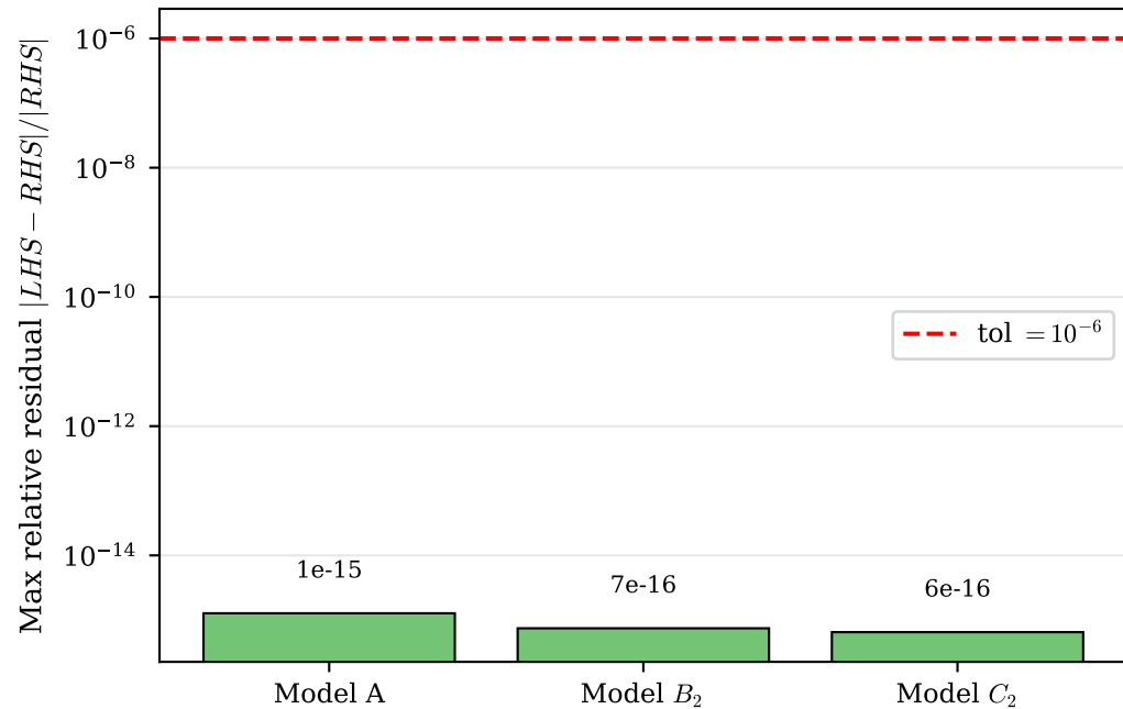
Lemma 2 — PPGF dynamics on \tilde{S}
