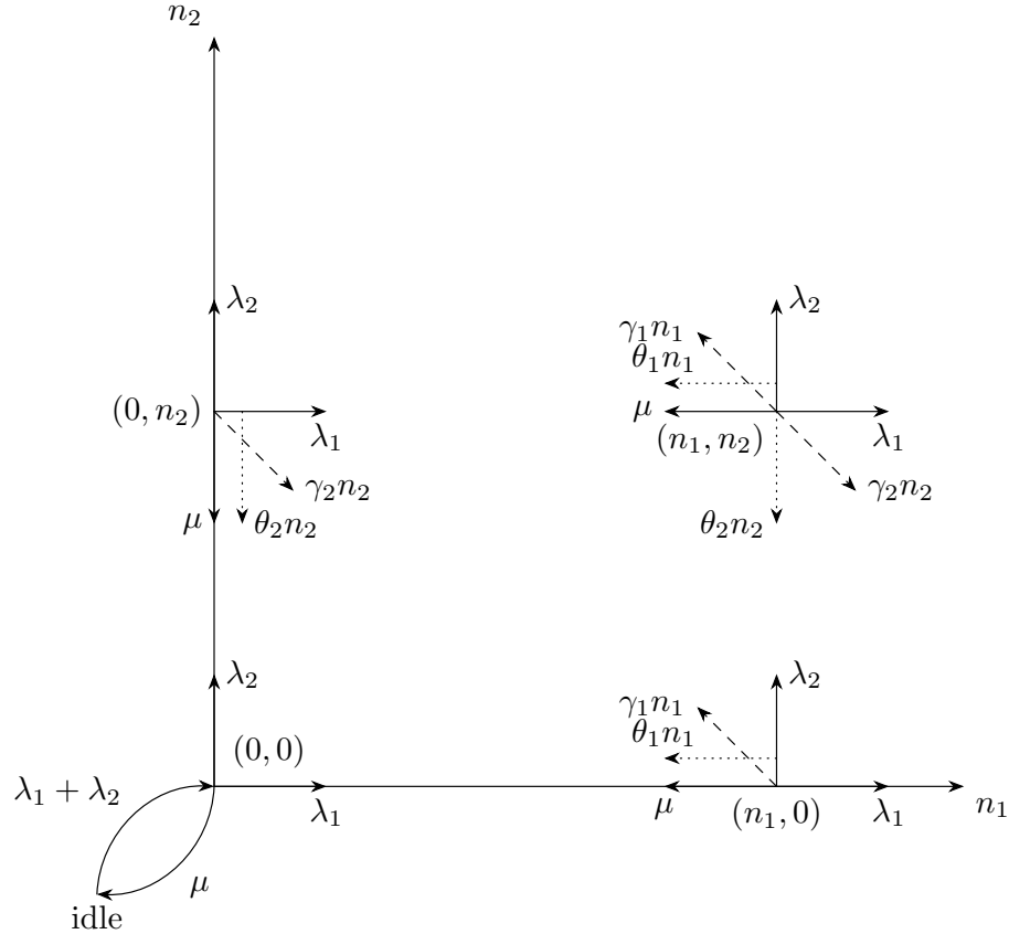
Figure 2: State transition diagram on state space S for the model with jockeying ( \gamma_i n_i , dashed) and abandonments ( \theta_i n_i , dotted).
