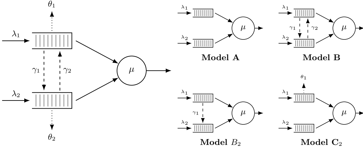
Figure 1: Physical queue layout for Model X (left) and its four specializations (right, 2 \times 2 grid). Queue 1 (top buffer) has non-preemptive priority over Queue 2. Solid arrows: Poisson arrivals ( \lambda_i ) and exponential service ( \mu ). Dashed arrows: jockeying ( \gamma_i ), which transfers a waiting customer between queues and conserves the total n . Dotted arrows: abandonment ( \theta_i ), a true departure that reduces n .
