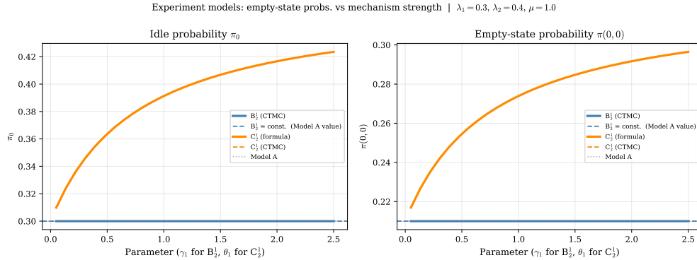
Figure 15: Empty-state probabilities \pi_0 and \pi(0,0) as the mechanism parameter increases from 0 to 2.5. Left : B_2^1 (blue) maintains \pi_0 = 1 - \rho exactly for all \gamma_1 — jockeying conserves total customers. C_2^1 (orange) shows \pi_0 increasing with \theta_1 : abandonment clears the priority queue faster, raising the server’s idle fraction. Right : same story for \pi(0,0) . Solid orange = closed-form formula (312); dashed orange = CTMC. The two are indistinguishable (max error < 10^{-4} ).
