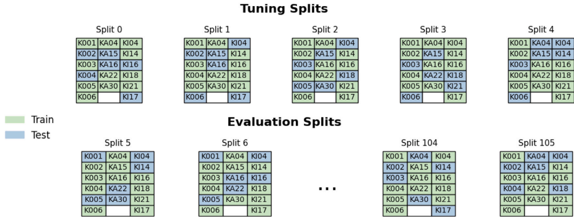
Fig. 5. Schematic of the Double Cross-Validation (CVM-CV) protocol applied to the PU dataset.
