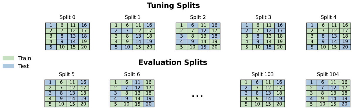
Fig. 4. Schematic of the Double Cross-Validation (CVM-CV) protocol applied to the UORED-VAFLS dataset. A distinct set of 5 bearing-level splits is used for hyperparameter tuning, while a separate set of 100 splits is used for final performance evaluation.
