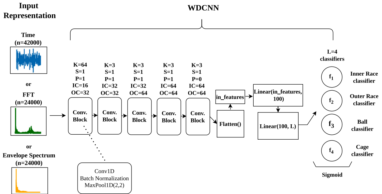
Fig. 8. Illustration of the proposed deep learning pipeline based on the WDCNN architecture, adapted for multi-label classification with L binary classifiers, with a choice of three possible input representations. For the UORED-VAFCLS dataset, input segments of length n = 42000 are used, with L = 4 outputs corresponding to the four fault modes present in the dataset. In the figure, each convolutional block is characterized by kernel size K , stride S , padding P , IC input channels, and OC output channels.
