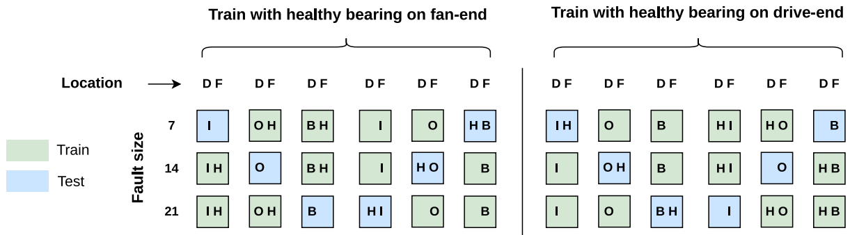
Fig. 7. Illustration of the proposed splitting methodology for the CWRU dataset. For each column, which represents bearings from a specific fault mode on a given location (e.g. column 1 represents inner-race fault bearings on the drive end), two faulty bearings are placed in the training set (green), while the remaining one is placed in the test set (blue). This figure also details two possible splitting scenarios that take into account the healthy bearings: training with healthy signals from the fan end (left panel) and training with healthy signals from the drive end (right panel). Green cells indicate signals used for training, whereas blue cells indicate signals reserved for testing.
