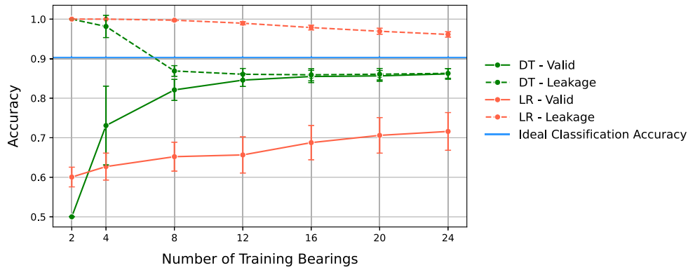
Fig. 1. Comparison of a low-capacity Decision Tree (DT) and Logistic Regression (LR) accuracy across varying numbers of training bearings, evaluated under two conditions: a leakage-free test (Valid) set and a test set with data leakage (Leakage). The higher-capacity LR appears to achieve higher performance under the data-leakage evaluation, even surpassing the theoretical optimal, which is an illusion caused by the fact that this evaluation is effectively a proxy for training performance.
