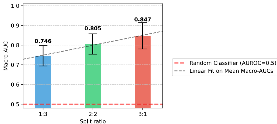
Fig. 20. Impact of train-test split ratio on model performance on the HUST bearing dataset using Random Forest with hand-crafted features.
