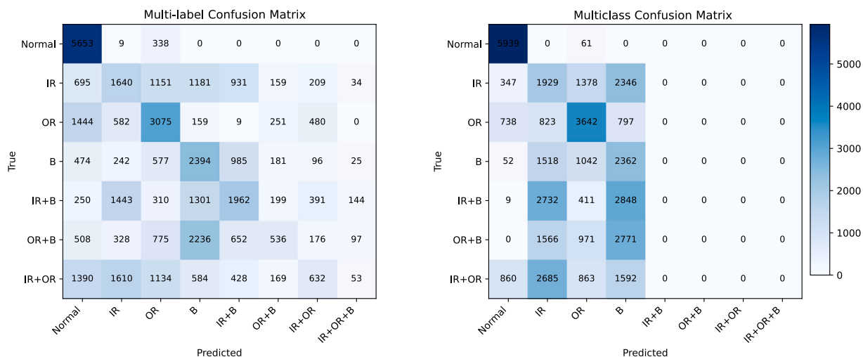
Fig. 19. Sum of confusion matrices obtained from models trained under the multi-label and multiclass frameworks on HUST bearing dataset. Each cell represents the sum of values across 100 train-test splits.
