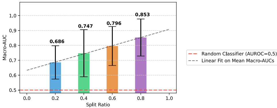
Fig. 12. Impact of train-test split ratio on model performance on the PU dataset using WDCNN with envelope spectrum as the input representation. In this figure, the N:M split ratio denotes N as the minimum number of bearings per class allocated to the training set, while M denotes the fixed number of bearings per class in the test set.
