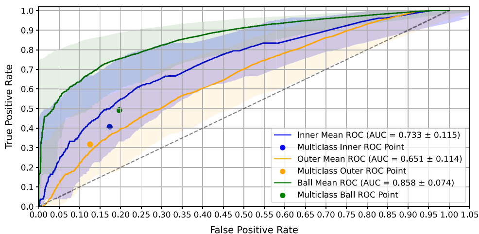
Fig. 18. ROC curves on the HUST bearing dataset using the (2:2, 0:2) split, where no co-occurring faults are present during training. The individual points represent TPR \times FPR mean values obtained from multiclass models when evaluated under a multi-label setup (independent binary fault classifiers)
