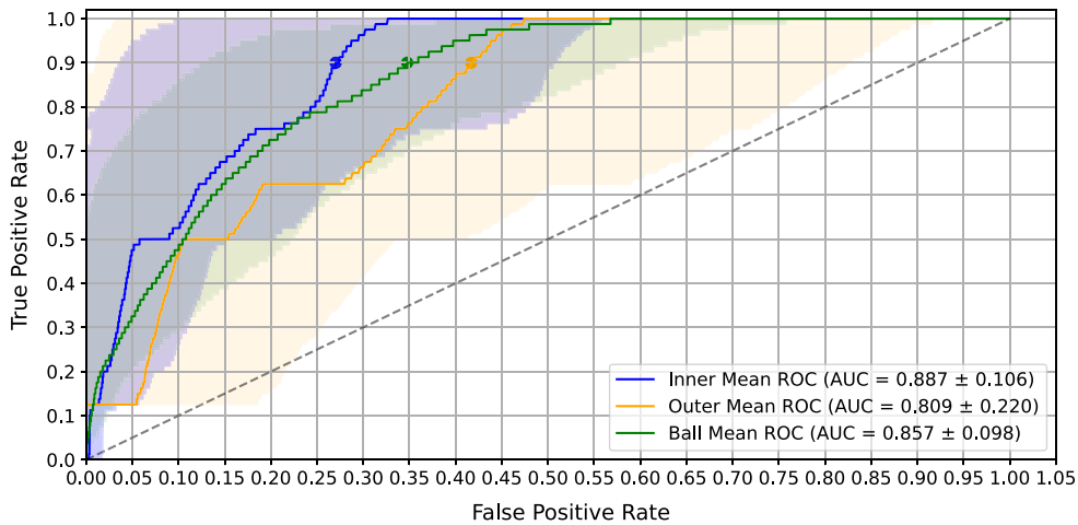
Fig. 13. ROC curves on the CWRU dataset for the Random Forest trained with handcrafted features. The solid curves represent the horizontal average across 100 runs, while, for each curve, the shaded region represents one standard deviation.
