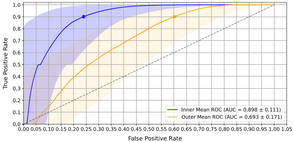
Fig. 11. ROC curves on the PU dataset for the WDCNN trained with envelope spectrum inputs. The solid curves represent the horizontal average across 100 runs, while, for each curve, the shaded region represents one standard deviation.
