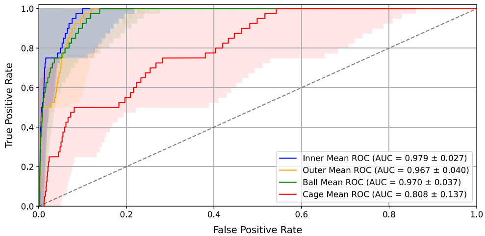
Fig. 9. ROC curves on the UORED-VAFCLS dataset for the frequency-domain WDCNN. The solid curves represent the horizontal average across 100 runs, while, for each curve, the shaded region represents one standard deviation.
