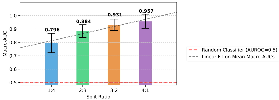
Fig. 10. Impact of train-test split ratio on model performance on the UORED-VAFCLS dataset. The plot shows the mean Macro AUROC (and standard deviation as error bars) calculated over 100 evaluation splits for four distinct bearing-level train-to-test ratios.
