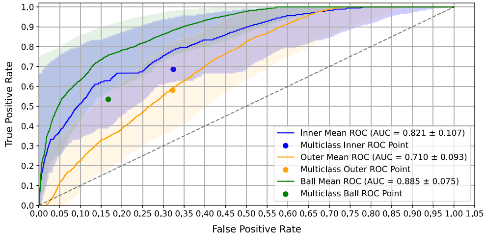
Fig. 17. ROC curves on the HUST bearing dataset for the Random Forest trained with handcrafted features on a 2:2 split. The individual points represent \text{TPR} \times \text{FPR} mean values obtained from multiclass models when evaluated under a multi-label setup (independent binary fault classifiers).
