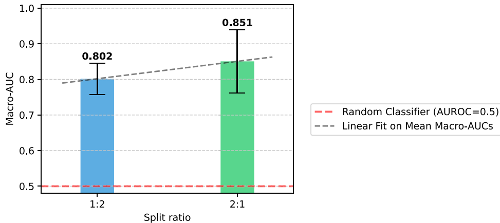
Fig. 14. Impact of train-test split ratio on model performance on the CWRU dataset using Random Forest with hand-crafted features.
