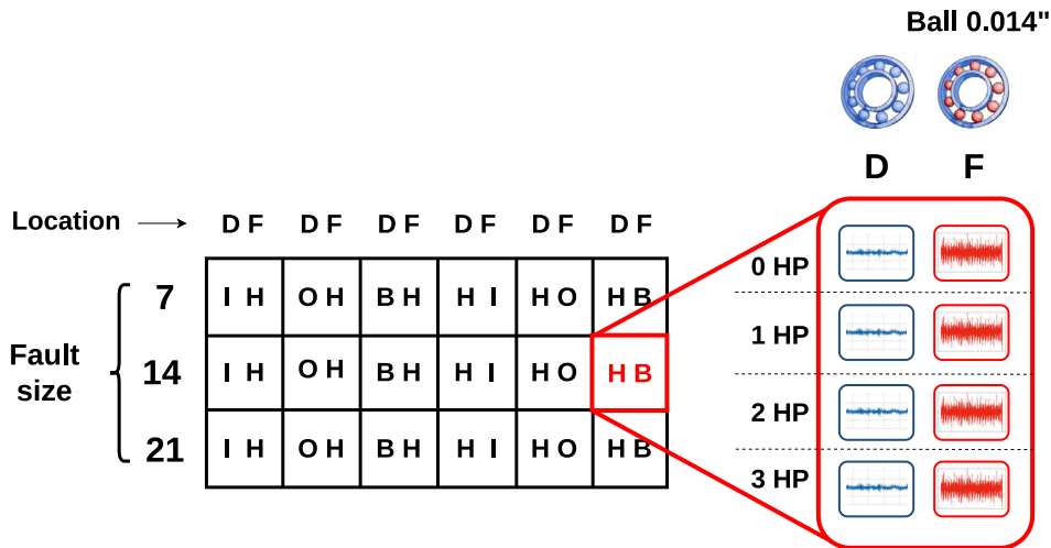
Fig. 6. Bearing configurations used in the CWRU dataset. Each cell represents a specific acquisition setup containing two bearings: one located at the drive end (D) and the other at the fan end (F). Fault types are denoted as follows: I for inner race fault, O for outer race fault, B for ball fault, and H for healthy.
