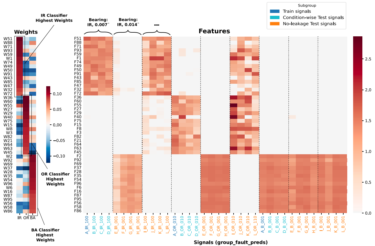
Fig. 16. Feature weight activation map for the WDCNN trained on Group A using time domain inputs from the CWRU dataset. The left panel displays the 45 most relevant classifier weights, obtained by selecting the 15 highest magnitude weights from each classification head (IR, OR, and BA). Rows labeled with W correspond to these classifier weights, grouped according to the classifier for which they are most relevant. The right panel displays the corresponding feature activations extracted by the model backbone for the same feature indices, allowing direct comparison between classifier importance and feature responses across signals. Rows labeled with F correspond to feature indices associated with the selected weights. The columns represent signals labeled according to Group FaultType Prediction , where each column denotes a specific group (A–L), fault mode (IR, OR, or B), and predicted output in the same order (e.g., “110” indicates a prediction containing both IR and OR faults). Bearings are arranged into groups of four columns, with each column corresponding to a different load condition. For example, signals associated with the bearing presenting an IR fault of size 0.007” are distributed across columns (A–D)_IR, whereas signals associated with the bearing presenting an OR fault of size 0.021” are distributed across columns (I–L)_OR. This visualization highlights how signals originating from the same bearing exhibit highly similar feature activation patterns, revealing the tendency of the model to memorize bearing specific signal characteristics rather than learn generalizable fault related predictors.
