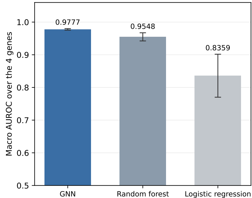
A. Like-for-like: the 4 genes the baseline fits in every seed
