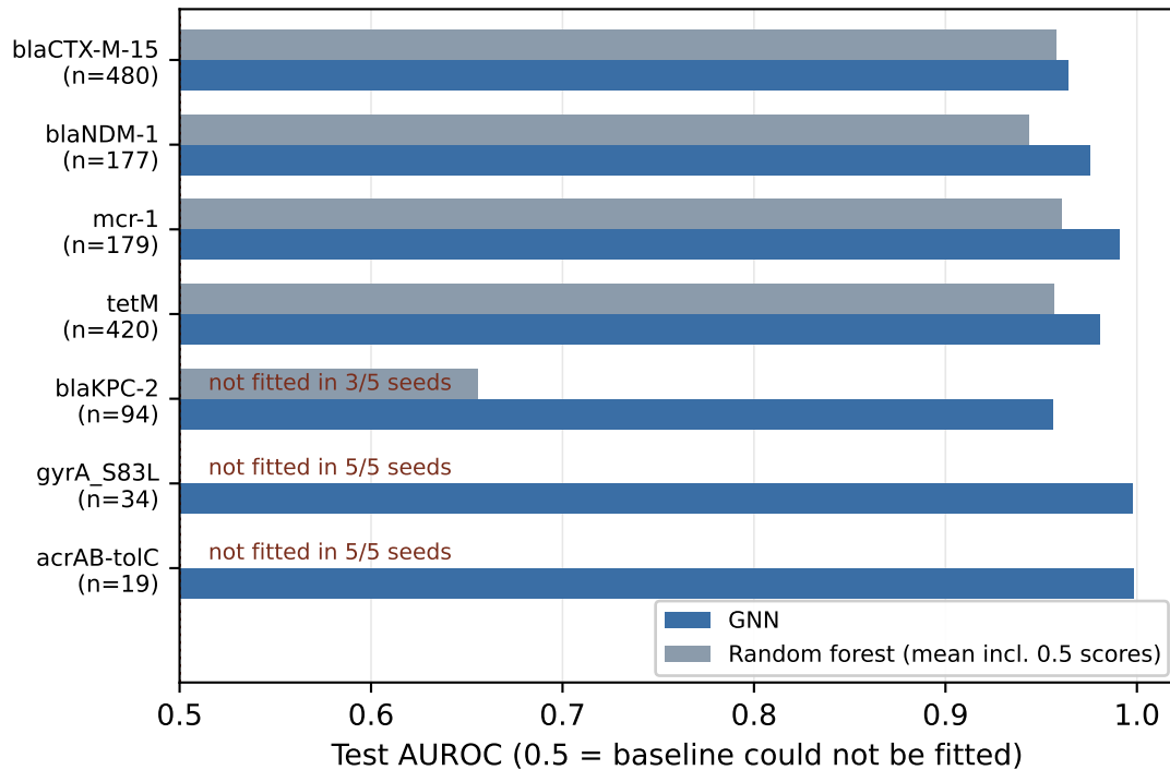
B. Per gene: where the per-gene baseline cannot be fitted at all
