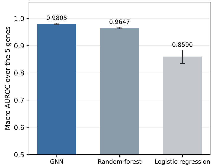
A. Like-for-like: the 5 genes the baseline fits in every seed
