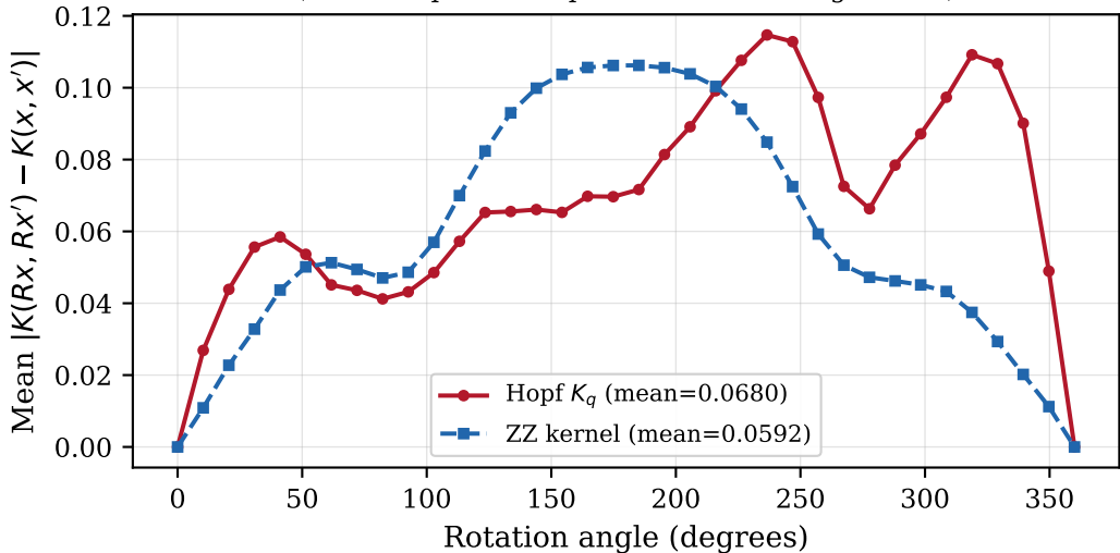
(d) Kernel Response to SU(2)-type Rotation (honest report: no equivariance advantage found)
