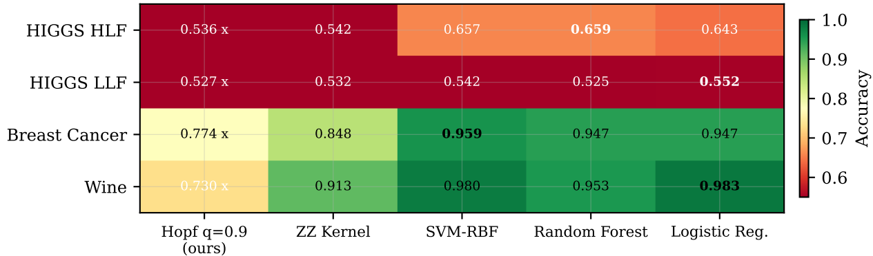
(d) Multi-dataset accuracy (classical methods shown as reference upper bound)
