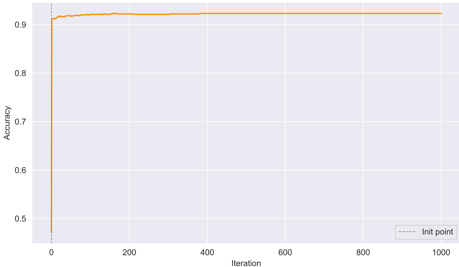
Task 2 – Training Accuracy vs. GD Iteration
