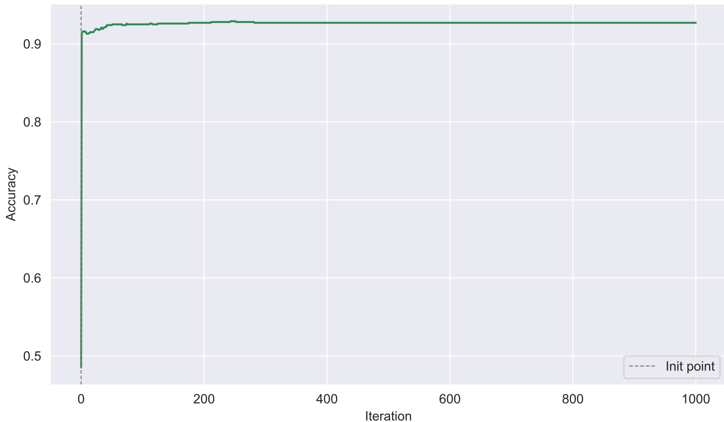
Task 2 – Testing Accuracy vs. GD Iteration
