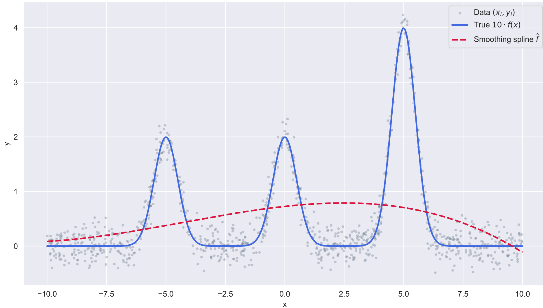
Task 3 (Image 2) – Smoothing Spline vs True Density Function
