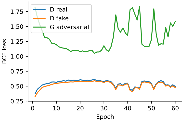
GAN adversarial terms
