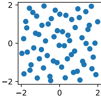
random grid (Sobol)
