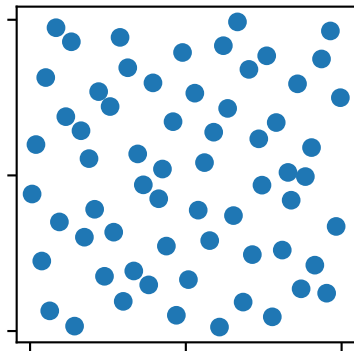
random grid (Sobol)
