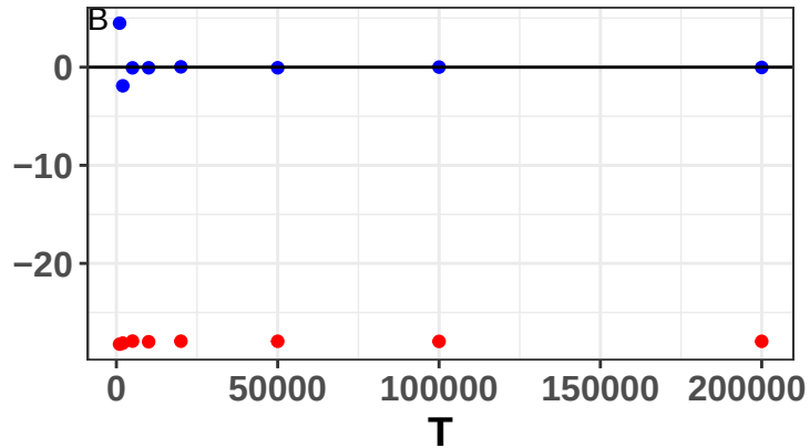
G=15 components, dimension of d=5
