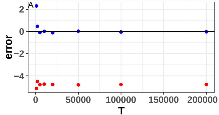
G=5 components, dimension of d=6
