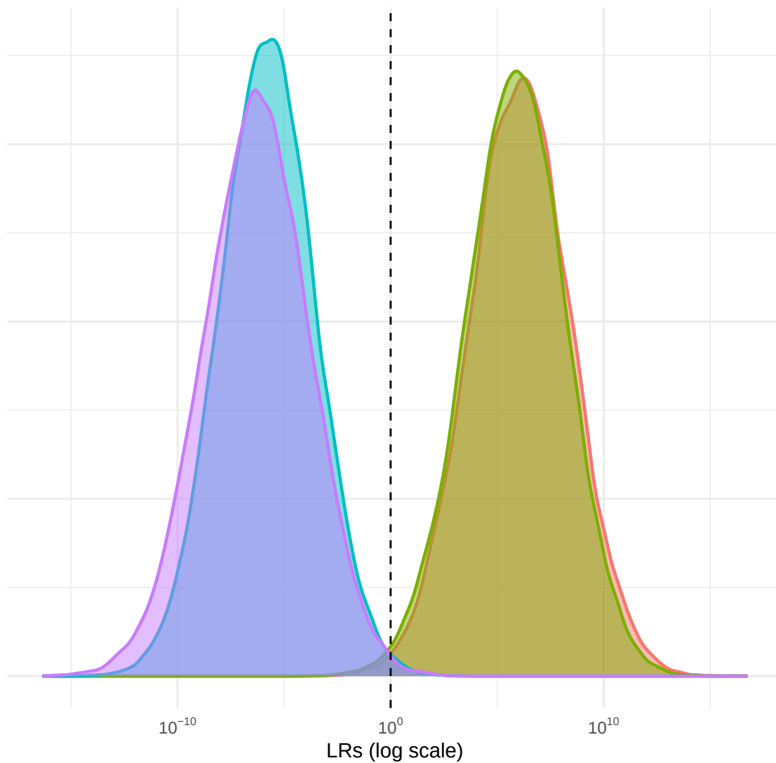
Distribution of LR s for Full Siblings vs Unrelated with 94 SNPs
