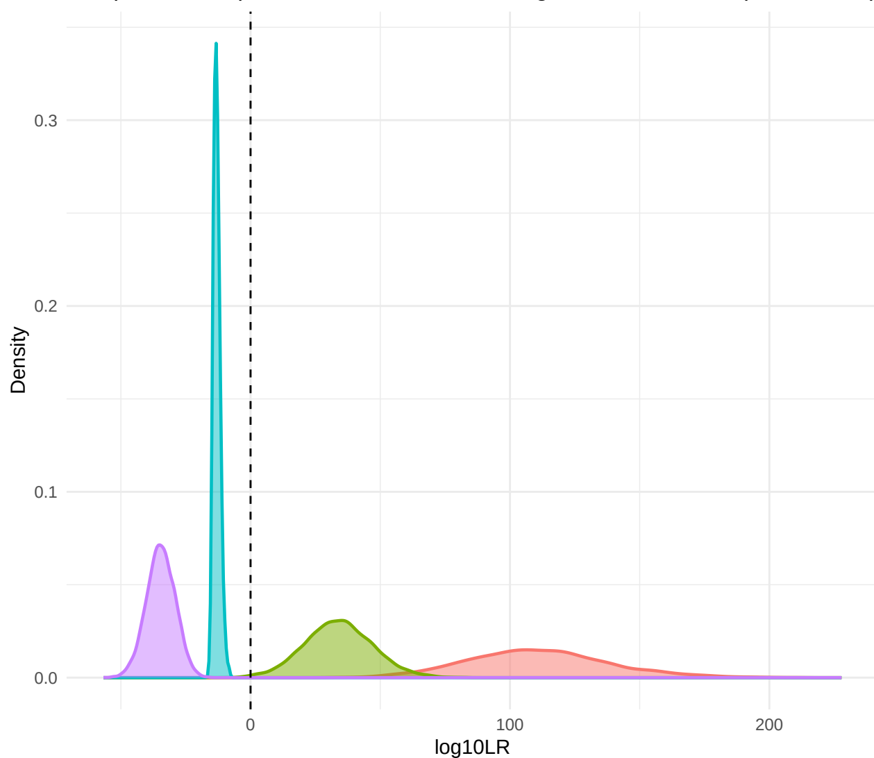
Independent Replication: FC vs UN – Full log10LR Distribution (9991 SNPs)
