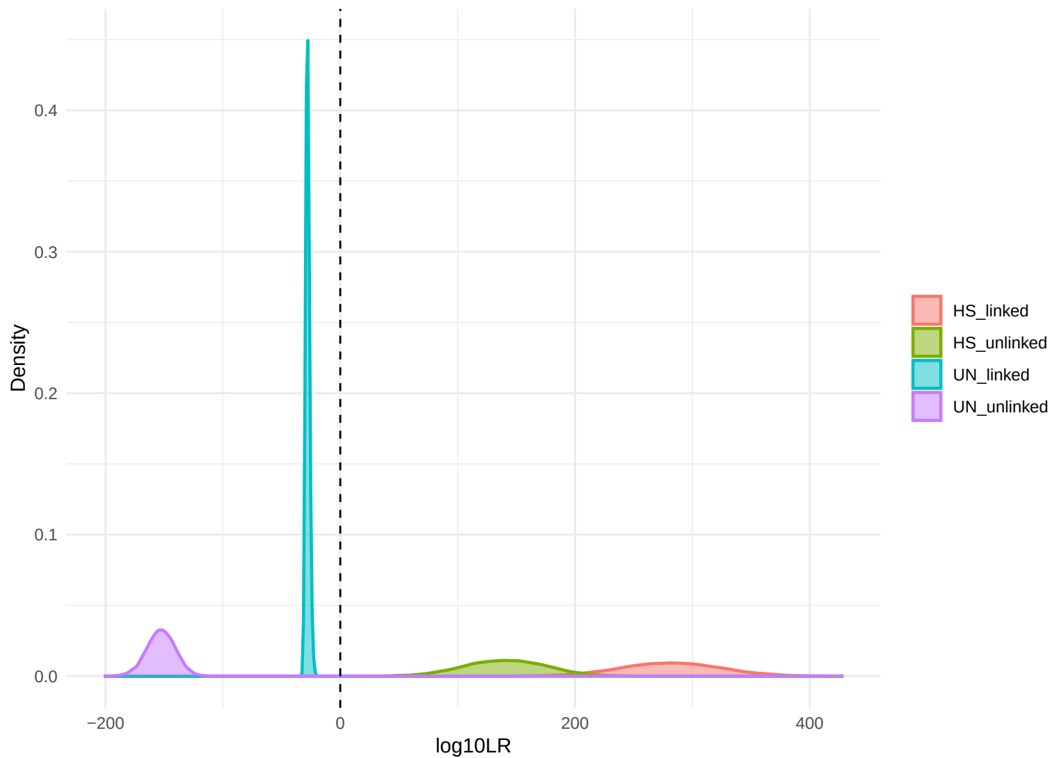
Independent Replication: HS vs UN – Full log10LR Distribution (9991 SNPs)
