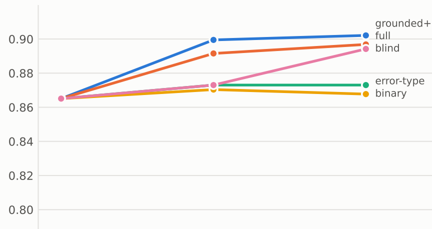
MBPP+ (single run)
