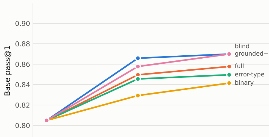
HumanEval+ (mean of 3 runs)
