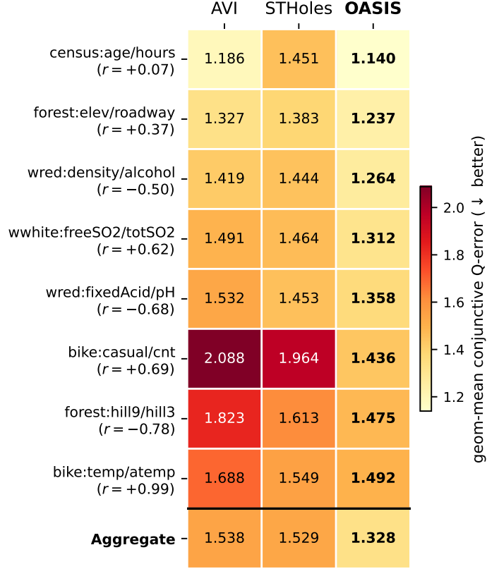
Fig. 3: Cross-column feedback repair on real correlated column pairs (rows ordered by |r| ): geometric-mean conjunctive-predicate Q-error (↓; paler is better), each cell annotated with its value, for independence with the true marginals (AVI), a faithful 2D STHoles [13] learned from the same K=16 conjunctive observations, and the OASIS feedback projection (2D max-entropy/IPF seeded from the marginals). OASIS is lowest on every pair; STHoles, lacking a maintained marginal, barely improves on AVI in aggregate ( 1.538 \rightarrow 1.529 ) and is worse than AVI on the weakly-correlated pairs, whereas OASIS reaches 1.328—a 13.6% aggregate reduction over AVI, concentrated where the columns are correlated.
