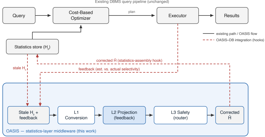
Fig. 2: OASIS as a statistics-layer middleware. The existing DBMS query pipeline (solid, top) is left unchanged. OASIS runs its own input-to-correction flow (solid): it reads the stale histogram H_0 and a recent feedback window, then applies conversion (L1), feedback projection (L2), and safety routing (L3) to emit a corrected histogram \hat{H} . It attaches to the pipeline only through the dashed integration hooks—tapping predicate feedback from the executor and substituting \hat{H} into the statistics the optimizer reads. All three layers are deterministic; L2 is the training-free feedback projection.
