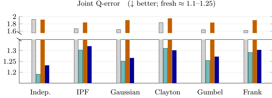
(a) Composition family (six estimators; dependence fixed, only the marginal varies): the projection (ISOMER, and OASIS, which coincides with it) recovers most of the stale joint Q-error, whereas the unprojected prior stays near stale.
