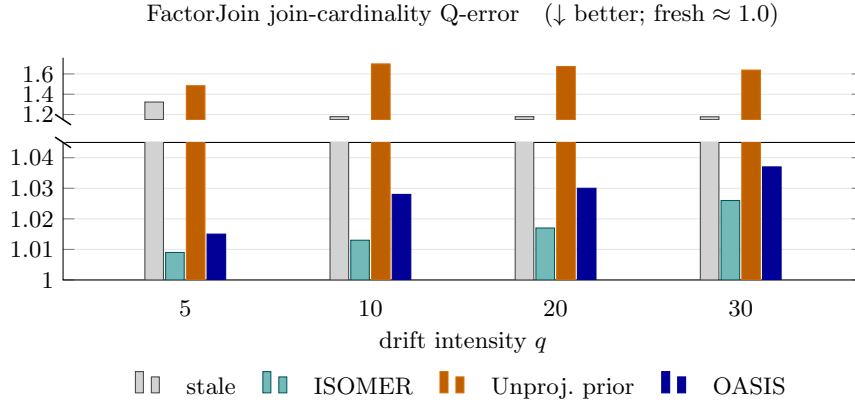
(b) FactorJoin bin-based join kernel as the join-key distribution drifts (only the single-column key histogram varies). The unprojected prior is actively harmful —its Q-error exceeds even stale, because the bilinear kernel amplifies mass-concentration errors—whereas the projected methods track the fresh marginal ( \approx 1.0 ).
