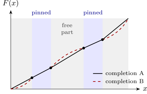
Fig. 1: Why feedback repair is underdetermined. A feedback window pins the cumulative mass F at the predicate boundaries it observes (dots); on the pinned intervals (blue) every consistent completion agrees, but on the regions the feedback leaves free (grey)—the free part—completions may differ (solid versus dashed) while still matching every observation—so the free regions are exactly what any repair method must fill, and once feedback pins them no choice remains (Section 4).
