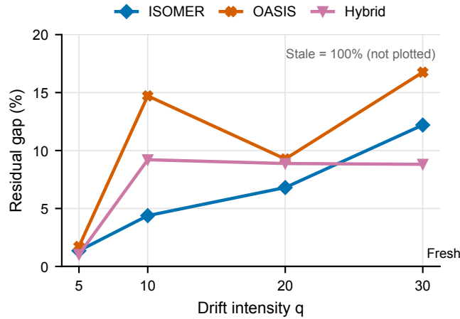
Fig. 1: FactorJoin join-cardinality Q-error by drift intensity for the deployed/calibrated marginal sources. Values are the residual gap to the fresh-marginal floor, normalized by the stale-to-fresh gap; 0% is fresh and 100% is stale, so lower is better.
