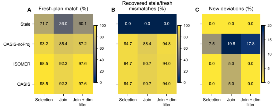
Fig. 2: PostgreSQL planner-only plan-shape effects by query family. Cell labels are percentages. Panel A reports fresh-statistics plan-shape match, Panel B reports recovery of stale/fresh mismatches, and Panel C reports new deviations where stale already matched fresh.
