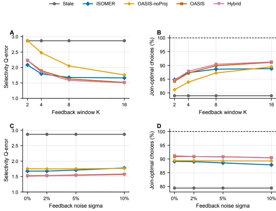
Fig. 3: Feedback-budget and feedback-noise sensitivity in the optimizer-decision proxy. Panels A–B vary the visible feedback window K ; Panels C–D perturb feedback selectivities with multiplicative log-normal noise while holding future predicates fixed. Dashed lines denote fresh statistics.
