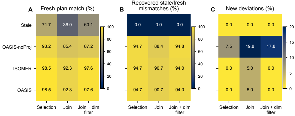
Figure 5: PostgreSQL planner-only plan-shape effects by query family. Cell labels are percentages. Panel A reports fresh-statistics plan-shape match, Panel B reports recovery of stale/fresh mismatches, and Panel C reports new deviations where stale already matched fresh.
