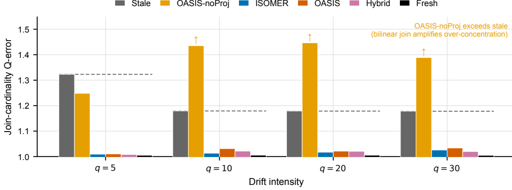
Figure 4: FactorJoin join-cardinality Q-error by drift intensity. Dashed lines mark the per-group stale baseline; arrows flag the regime where OASIS-noProj exceeds stale. In the bilinear join kernel, the uncalibrated learned marginal (OASIS-noProj) is harmful for q \geq 10 , whereas the full OASIS and Hybrid stay at the fresh-marginal floor.
