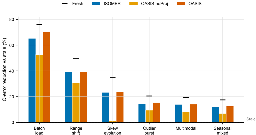
Figure 3: Out-of-distribution drift families: percentage reduction in geometric-mean selectivity Q-error relative to stale (higher is better; black ticks are the fresh reference). The projected OASIS matches or edges ISOMER on every unseen family, while the raw OASIS-noProj over-extrapolates—collapsing to near zero on skew evolution. The prior is trained only on the domain-randomized mixture. Values from Table 8.
