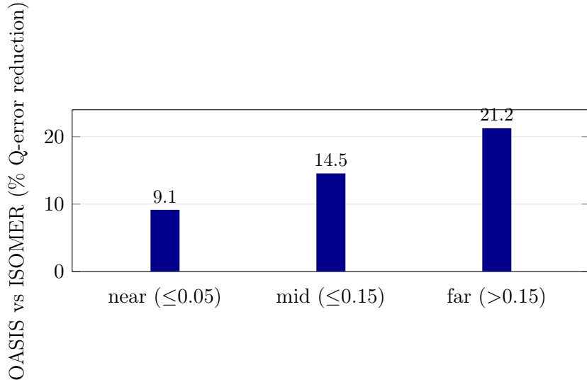
Figure 2: The learned completion’s advantage over ISOMER grows monotonically with a held-out predicate’s distance from the nearest feedback endpoint—the spatial signature of a nullspace completion. Near feedback, where the projection already pins the marginal, the gain is 9.1%; far from any feedback, squarely in the nullspace, it is 21.2%. Values from Table 4.
