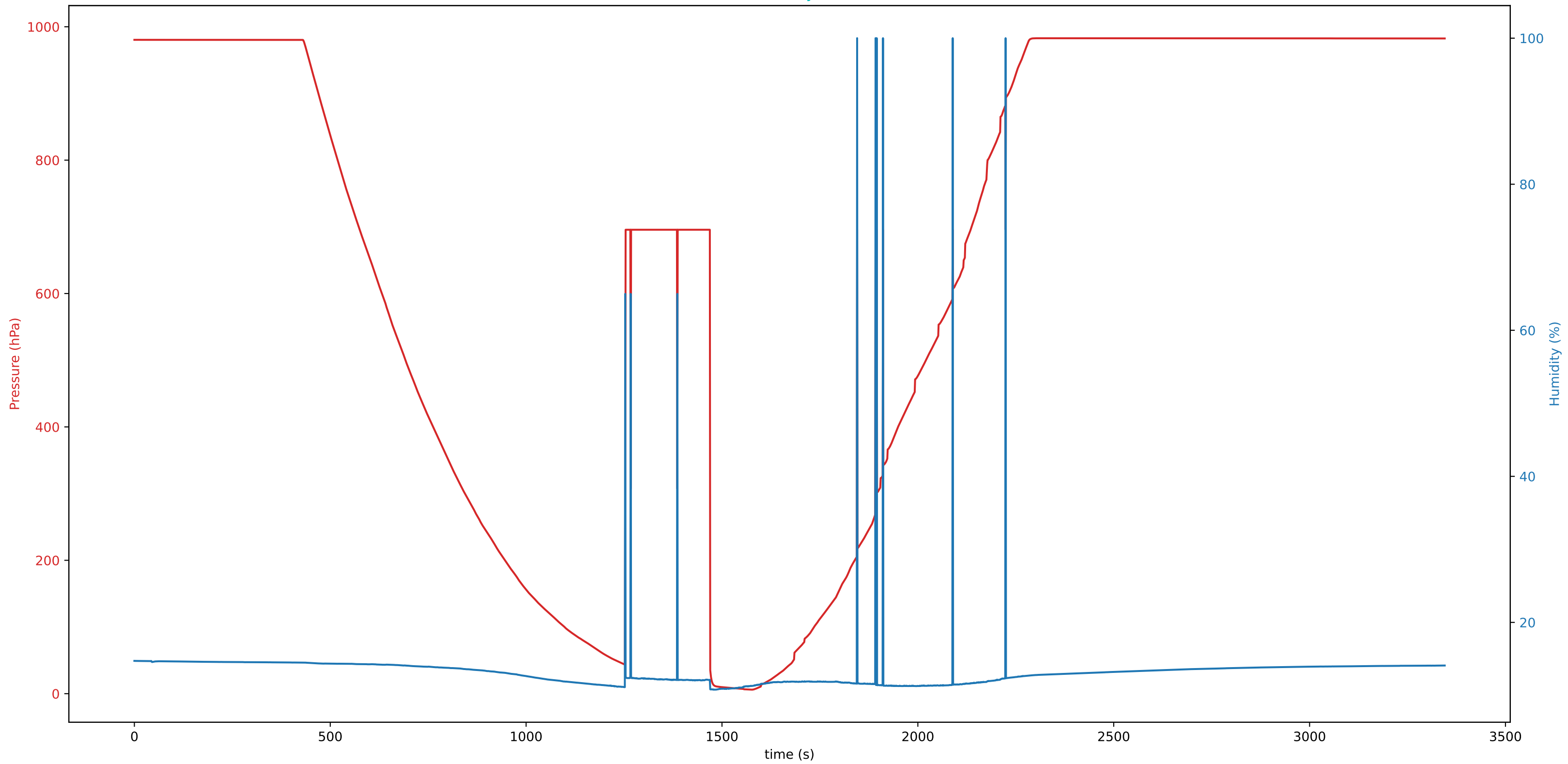
LX-179-A Humidity vs Pressure
