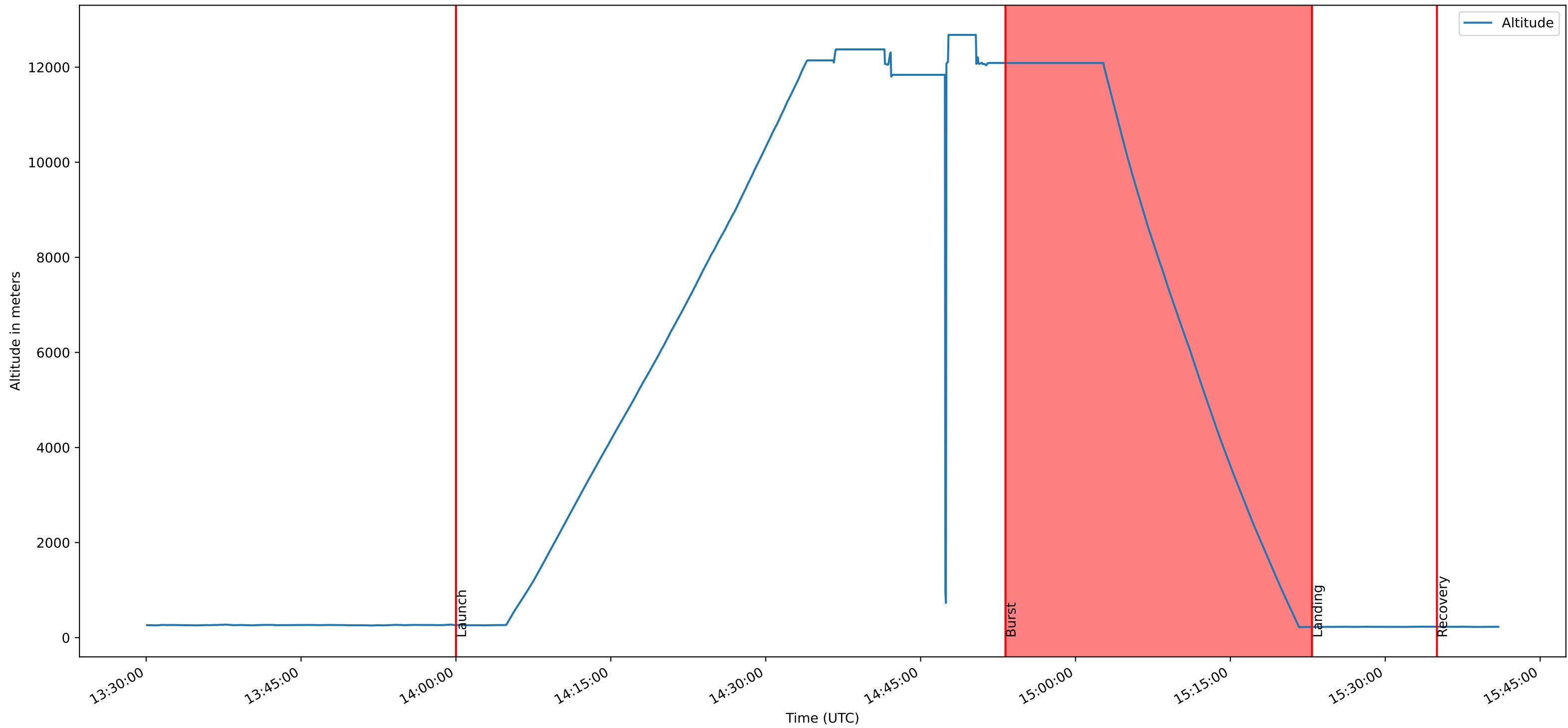
LX-179-B Altitude Plot
