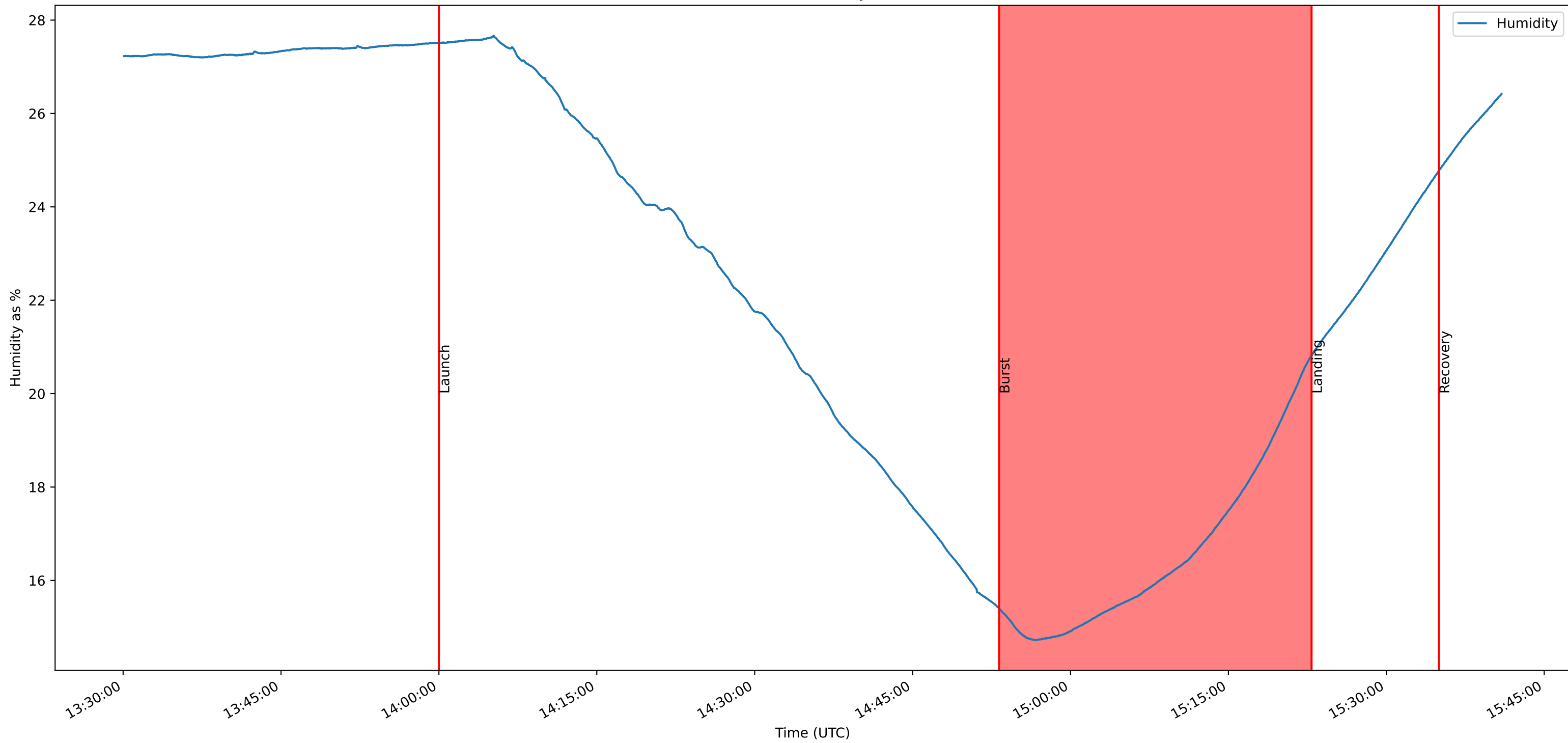
LX-179-B Humidity Plot
