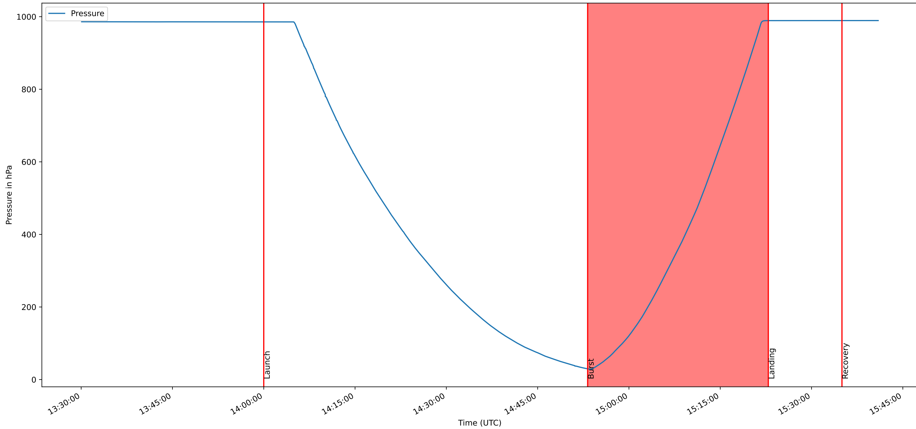
LX-179-B Pressure Plot
