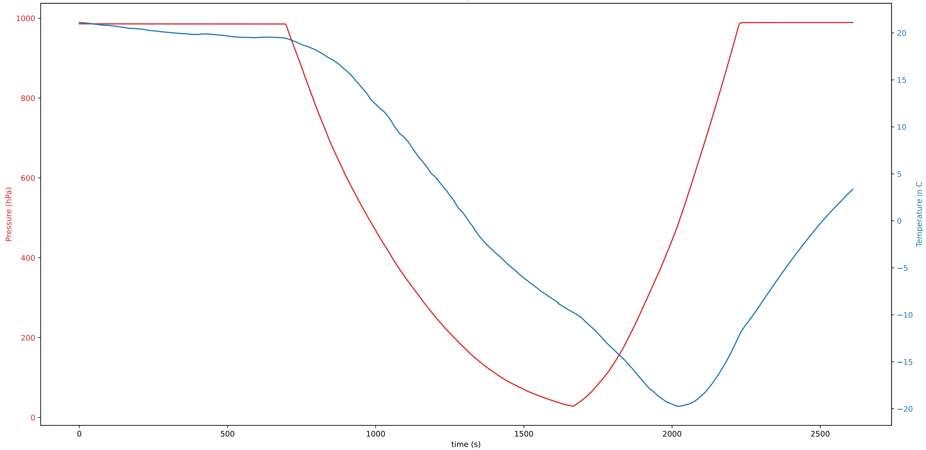
LX-179-B Temp vs Pressure
