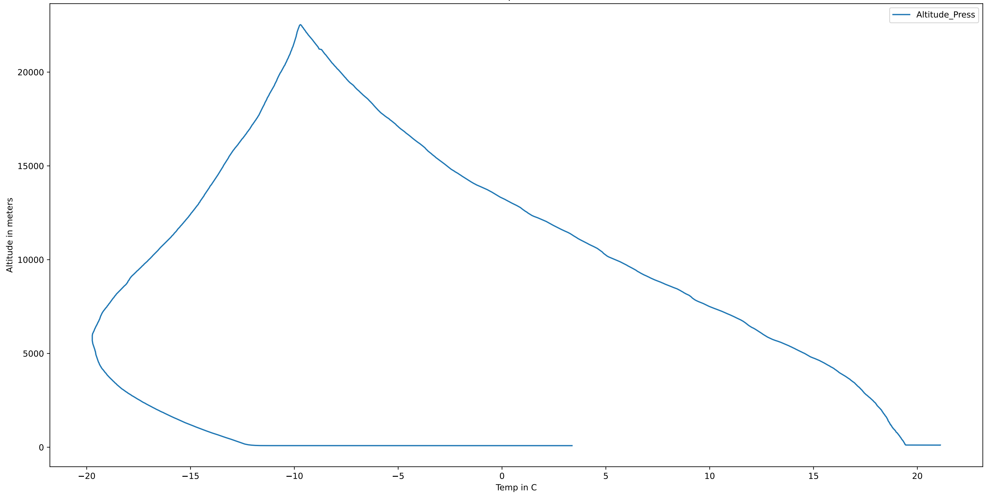
LX-179-B Temp vs Altitude Plot
