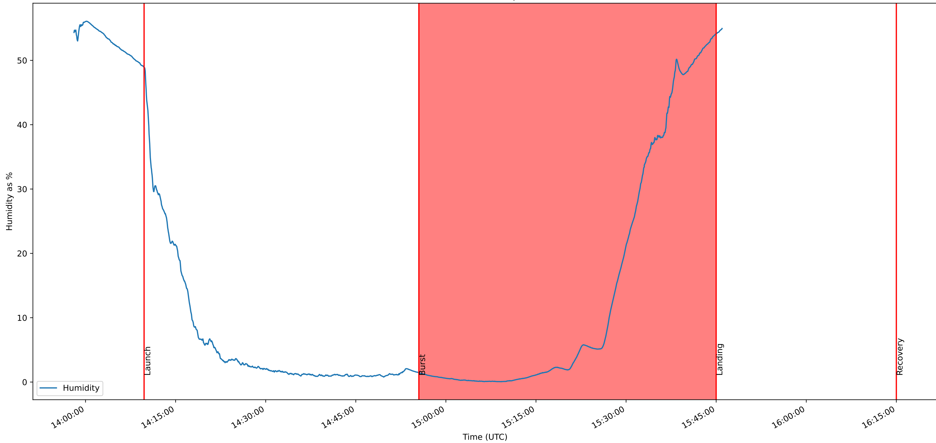
LX-187-B Humidity Plot
